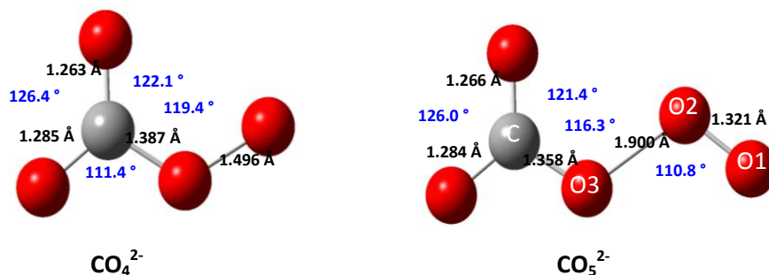
Figure 2: Optimized structures of \text{CO}_4^{2-} and \text{CO}_5^{2-} at the B3LYP/6-31G (d) level.
