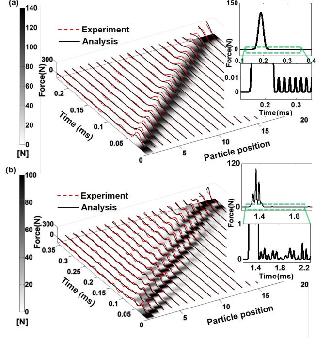
FIG. 2: Numerical (solid black) and experimental (dashed red) force profiles in space-time (measured in ms) in 1D woodpile crystals composed of (a) 20 mm and (b) 40 mm rods. The insets show the numerical magnified force profiles of nanoptera, while the colormap represents the magnitude of the contact force.
