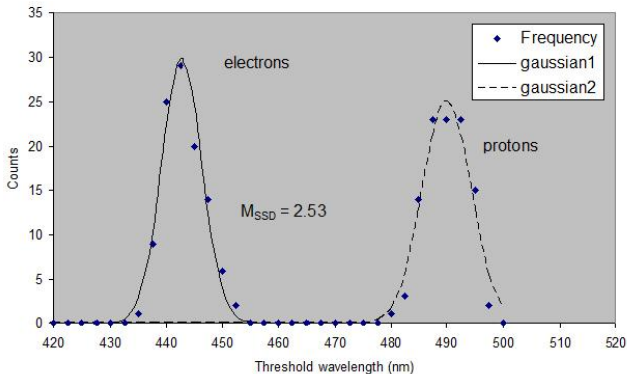
Figure 21. Spectral-shape discrimination histogram derived from steady-state radioluminescence data of DUT-6 infiltrated with \text{Ir}(\text{ppy})_3 .
