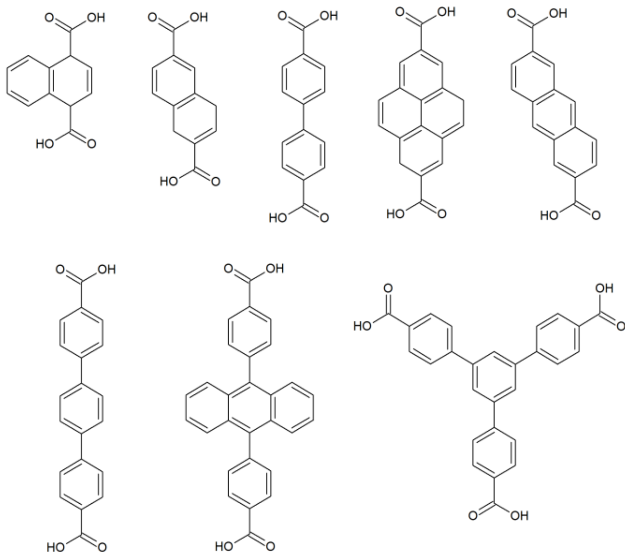
Figure 2. Carboxylic acid linker groups employed in this study.
