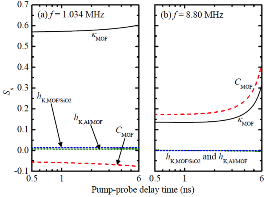
Figure S3. Sensitivities of the TDTR signal (ratio of in-phase to out-of-phase voltages recorded by the lock-in amplifier, -V_{\text{in}}(t)/-V_{\text{out}}(t) ) to various thermophysical properties in the sample x , where x denotes \kappa_{\text{MOF}} , C_{\text{MOF}} , h_{\text{K,Al/MOF}} or h_{\text{K,MOF/SiO}_2} . These sensitivities were calculated via Eq. S1 assuming a pump modulation frequency of (a) f = 1.034 MHz and (b) f = 8.80 MHz.
