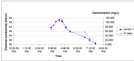
Figure 3. Electronic conductivity and concentration values of sensor 1
