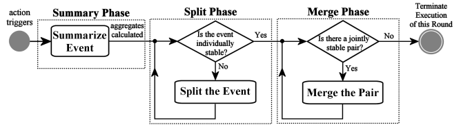
Figure 5. Algorithm phases of DRAGON
