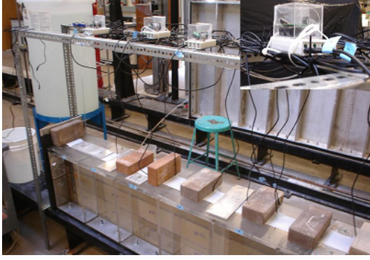
Figure 2. An intermediate scale tank instrumented with motes and conductivity probes
