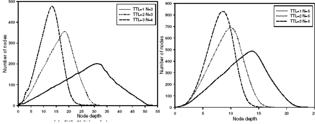
Figure 4. Number of nodes at different levels of the cluster tree for breadth first tree formation. Left: Simple hierarchical clustering scheme (SHC); and Right: Hierarchical hop-ahead clustering (HHC).
