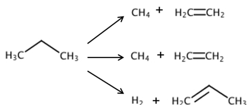
Scheme 2. Reaction network for propane cracking and dehydrogenation. The appearance of only one type of C-C bond leads to only one product (CH 4 /ethylene) from cracking. Dehydrogenation of propane leads to the formation of propylene and H 2 .
