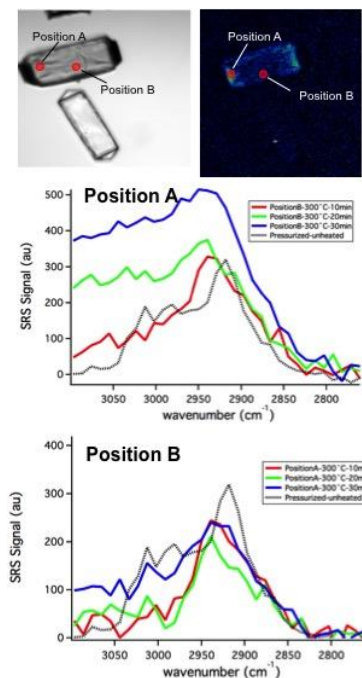
Figure 10. Transmission and SRS images at 300°C with locations marked for where spectra were generated.
