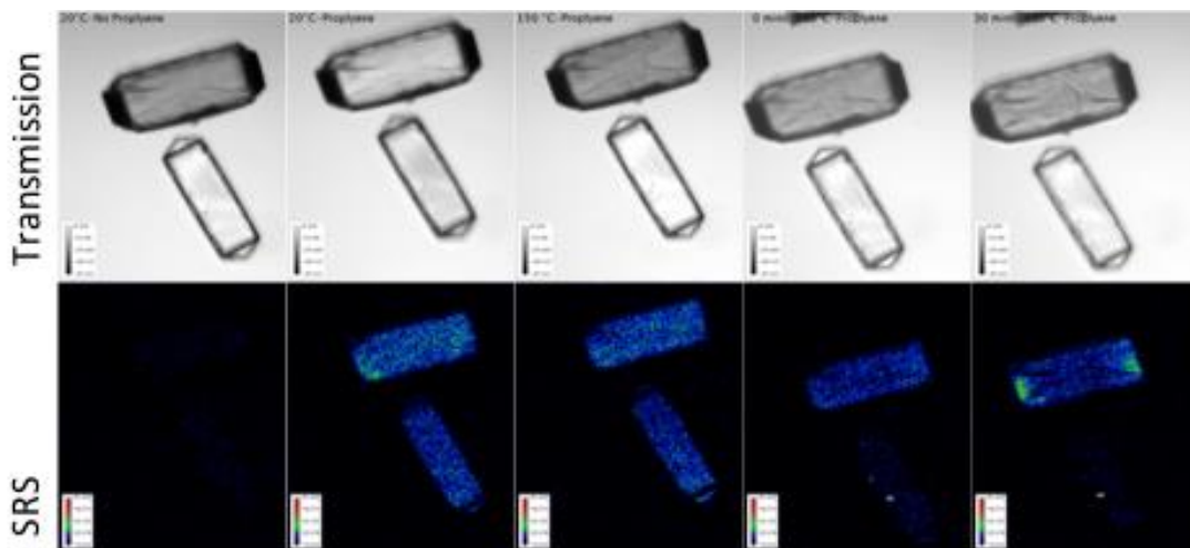
Figure 9. Transmission and SRS images of single-body MFI exposed to propylene and then heated to 300 °C.
