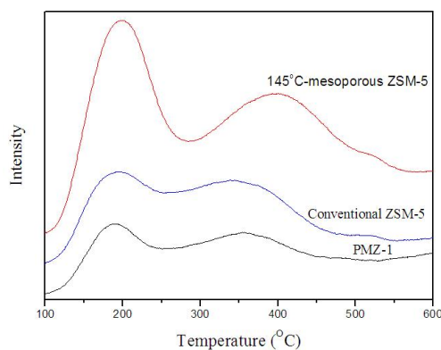
Figure 20. Ammonia TPD profiles for PMZ-1, a conventional ZSM-5, and 145^\circ\text{C} -M-ZSM-5. The profiles confirm the presence of both strong and weak acid sites in the PMZ-1 and hierarchically mesoporous MFI zeolite obtained after hydrothermal treatment at 110^\circ\text{C} and 145^\circ\text{C} for 48 h, respectively. The results demonstrate that PMZ-1 has an acidity similar to the conv-MFI zeolite.
