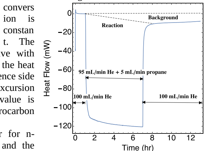
Figure 15. DSC measured heat flow as a function of time-on-stream during propane dehydrogenation. It is apparent that the measured heat flow has not reached steady-state even after five hours.
