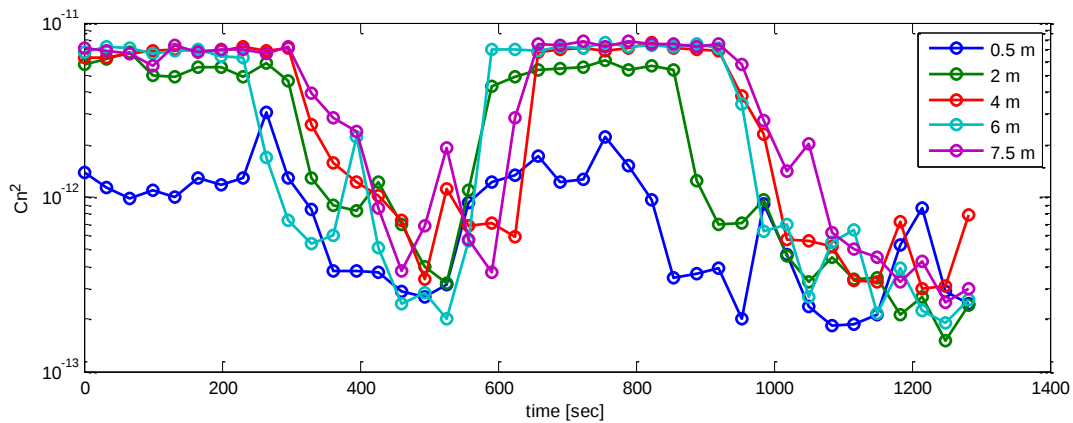
Figure 10 The measured C_n^2 values as a function of time with the on-off-on-off pattern of the space heater for different positions of the space heater as measured from the FMCW ladar Tx/Rx aperture.
