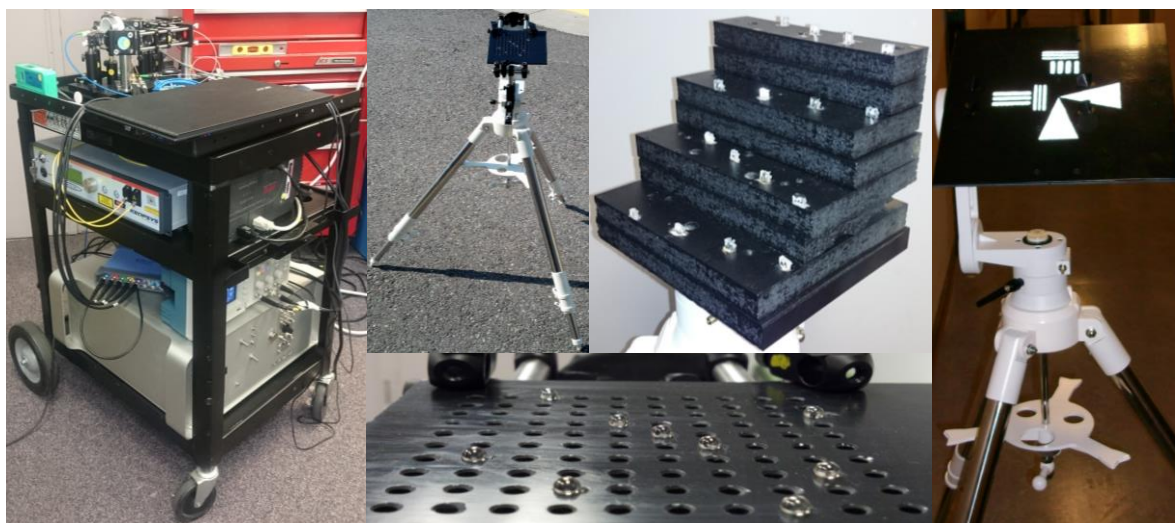
Figure 6 Portable ranging/imaging system and target system on tripod with gridded ball retro targets and a target pattern constructed of retro-reflecting tape for SAL and DSAL studies.
