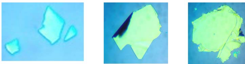
Figure 60. Locating NbSe 2 2-D crystals with the contrast method.
