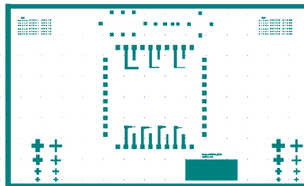
Figure 39. Metallization mask.
