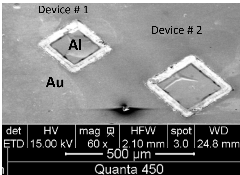
Figure 43. Top-down scanning electron microscope (SEM) image of a constructed Al/ \text{AlO}_x /Al device as shown in the schematic in Figure 36.
