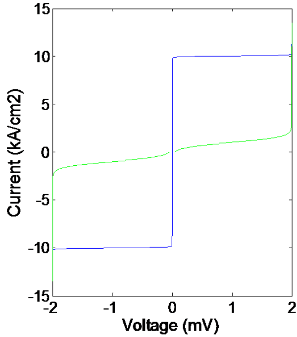
Figure 27. Modeled (hysteretic) forward and reverse characteristics representative of a quantum memory device.
