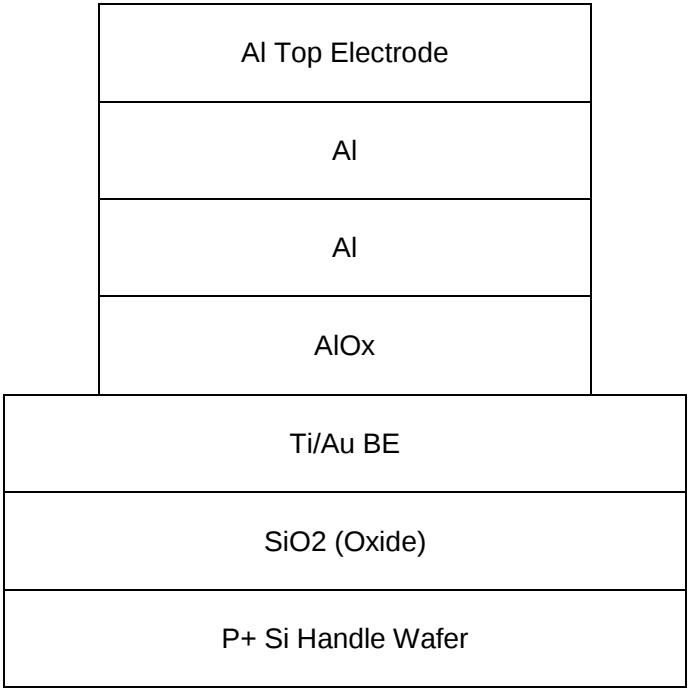
Figure 42. Cross-section schematic of constructed Al/AlO x /Al devices.
