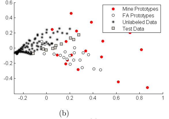
Figure 6. Illustration of the advantage of using additional unlabeled samples in detecting targets. (a) a sample target and the confidence values assigned at each of the 10 depths by LP10 and LP with more unlabeled data. (b) Scatter plot of the target/non-target prototypes, test samples at the 10 depth bins, and additional 30 unlabeled samples. Here the 16 dimensional feature space is projected into 2-D using multi-dimensional scaling.
