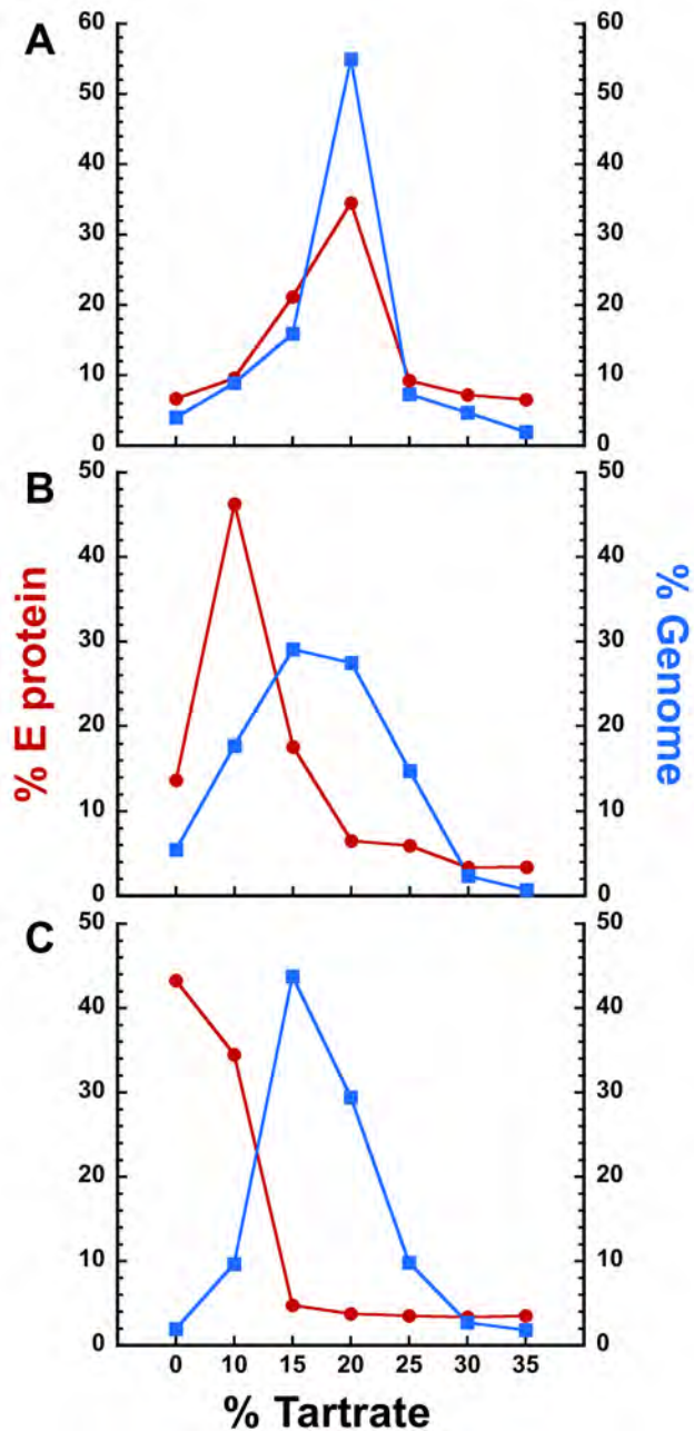
Figure 1: The E protein and genome of virus particles can be separated in a density gradient following treatment with DN59.
