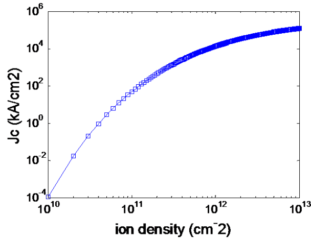
Figure 21. J_c vs. ion density.
