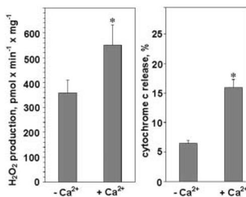
Fig. 4 \text{Ca}^{2+} -induced cytochrome c release and stimulation of \text{H}_2\text{O}_2 production by brain mitochondria oxidizing succinate. Mitochondria were added at a concentration of 0.25 mg/mL to the standard incubation medium maintained at 37°C and supplemented with 5 mM succinate. As in Fig. 2, approximately 3 min later, rotenone (0.2 \mu\text{M} ) was added, followed 2 min later by either \text{Ca}^{2+} (0.2 mM) or vehicle control ( \text{H}_2\text{O} ). The rate of \text{H}_2\text{O}_2 production was determined by the rate of increase in Amplex Red fluorescence. At approximately 8 min following the addition of \text{Ca}^{2+} , the suspension was centrifuged and the pellet and supernatant fractions used for ELISA of cytochrome c content, as described in Materials and Methods. Values represent the mean \pm SE of four independent experiments. * p < 0.05 versus without \text{Ca}^{2+} by Student's t -test.
