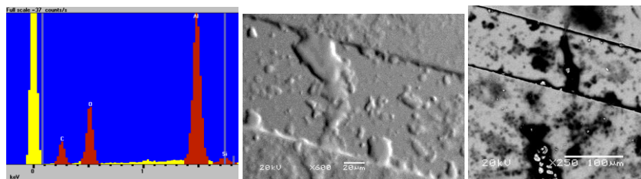
Figure 5: Evidence of contamination by carbon of all exposed samples was confirmed by analyses at UIUC. The figure on left clearly shows a carbon peak (red, labeled “c”) from an SEM-EDXS image of an alumina \text{Al}_2\text{O}_3 tile exposed to plasma. Figure in the right and on the right are back scattered electron (BSE) images of exposed silicon (center right). Note accumulation of carbon in topographical image (center) and prevalence of black, indicative of carbon on right image.
