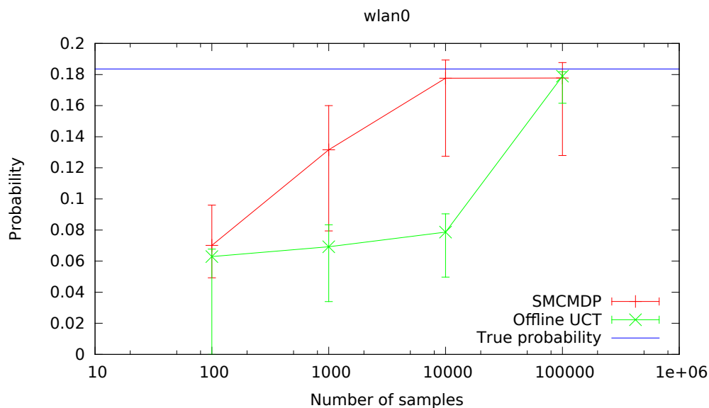
Figure 4: Probability estimates from SMCMDP on a WLAN model, the averaged over 100 runs.
