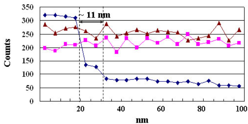
Fig. 3.6. (a) EDXS profile along line arrowed in Fig. 3.5 (a); and (b) EDXS profile along line arrowed in Fig. 3.5 (b).
