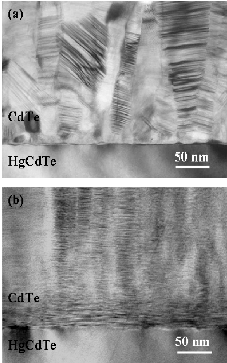
Fig. 3.2. Cross-sectional electron micrographs comparing the typical microstructure of CdTe capping layers deposited by: (a) HWE; and (b) MBE.
