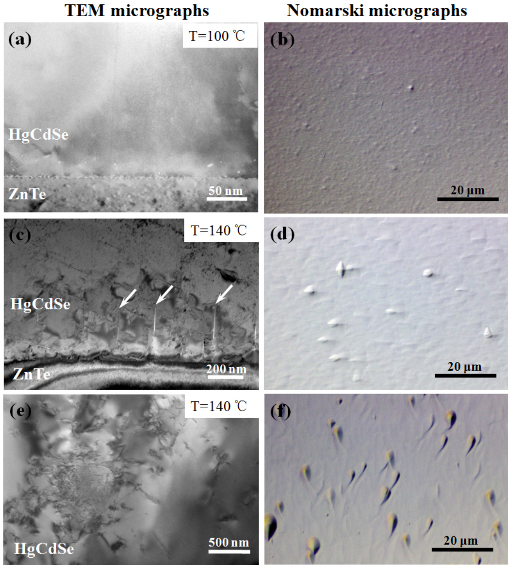
Fig. 5.1. (a), (c) and (e): cross-sectional electron micrographs of \text{Hg}_{1-x}\text{Cd}_x\text{Se}/\text{ZnTe}(112) heterostructure grown at T=100^\circ\text{C} , 140^\circ\text{C} and 140^\circ\text{C} ; (b), (d), and (f): Nomarski optical images of the corresponding \text{Hg}_{1-x}\text{Cd}_x\text{Se} surface.
