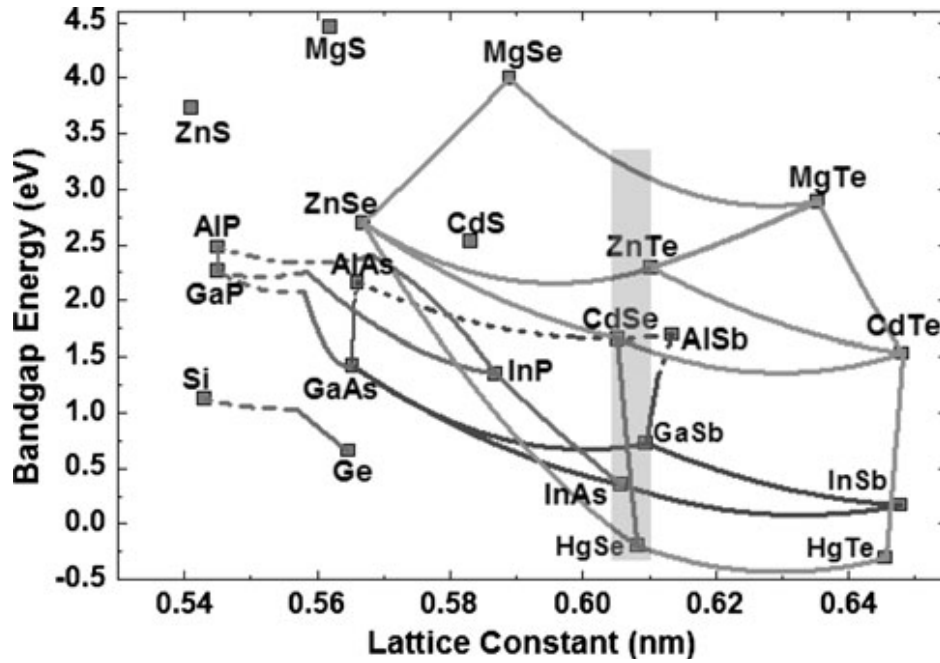
Fig. 1.8. Energy gap versus lattice parameter for several semiconductor material systems. The shaded region highlights semiconductors that have lattice parameters near 6.1Å. 27
