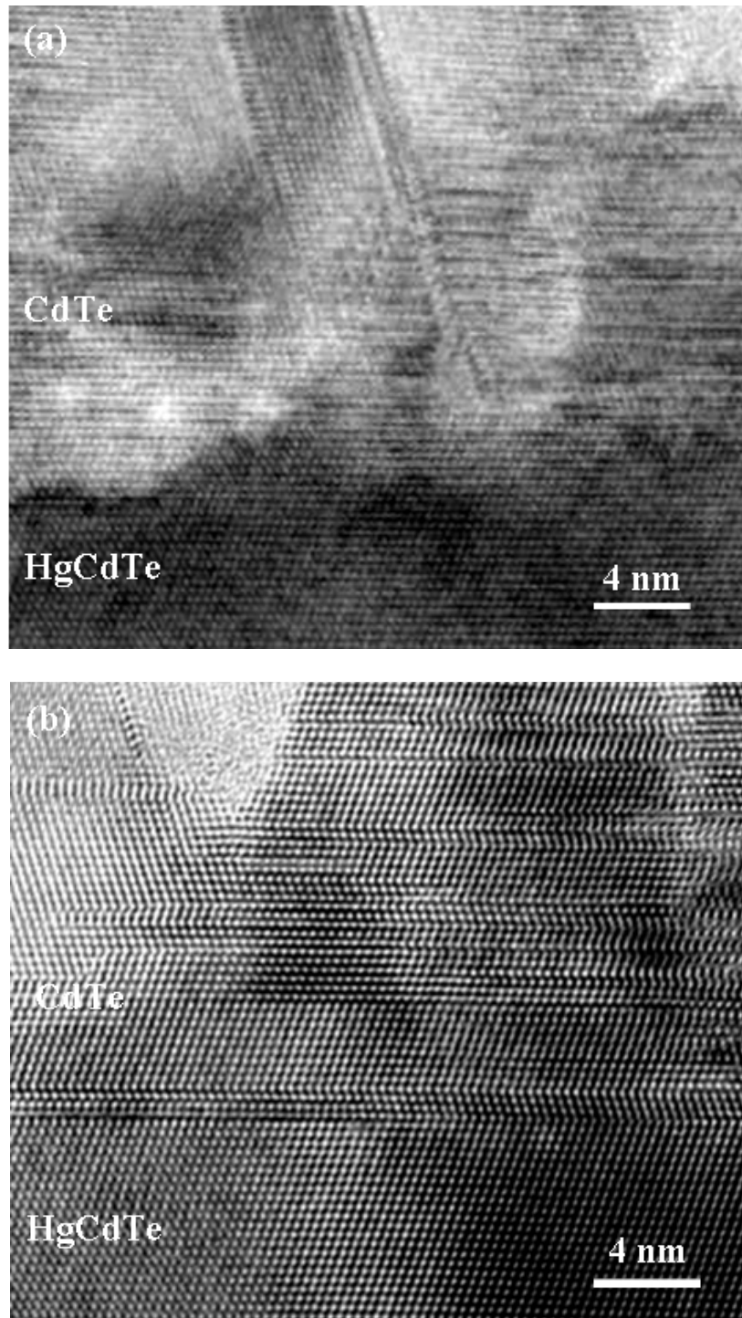
Fig. 3.4. High-resolution electron micrographs comparing flatness of CdTe/HgCdTe interface: (a) before annealing; and (b) after annealing.
