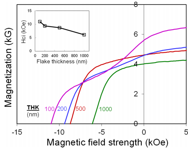
FIG. 5. Demagnetization curves of \text{SmCo}_5 bulk samples pressed at 600^\circ\text{C} and 420\text{ MPa} with different thickness flake powders; the bulk coercivity as a function of flake thickness (inset).
