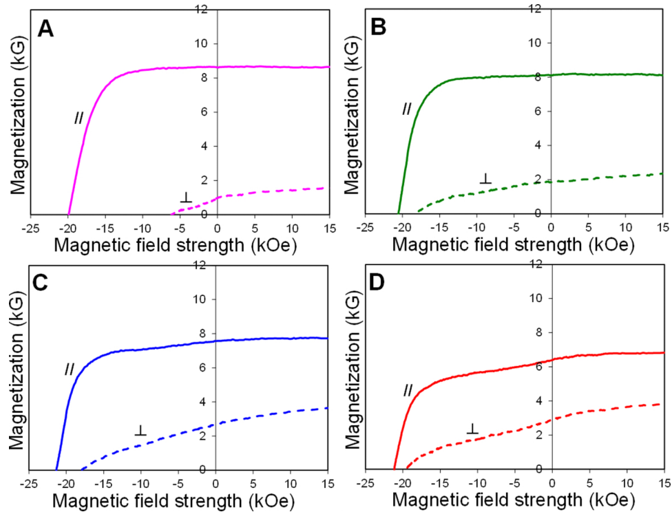
FIG. 4. Demagnetization curves of aligned flake powder samples measured along parallel ( \parallel ) and perpendicular ( \perp ) to the aligning magnetic field direction with flake thickness of A) 1000 nm; B) 500 nm; C) 200 nm; D) 100 nm.
