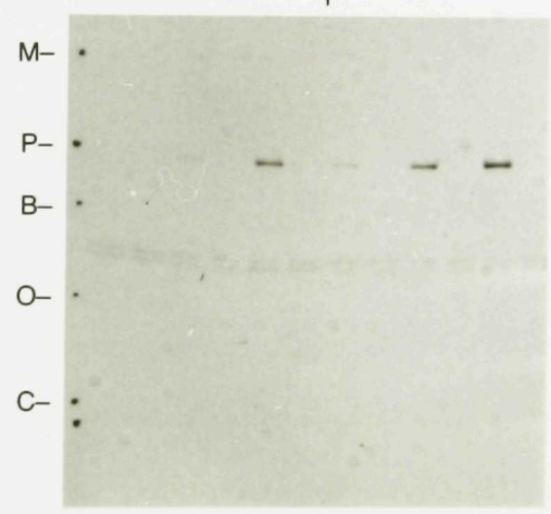
Fluorograph of [ 3 H] Dex-Mes Labeled Receptors C) Unactivated Activated Std NI AP BU NI AP BU [ 1 H] Dex - + - + - + - + - + - + - +
