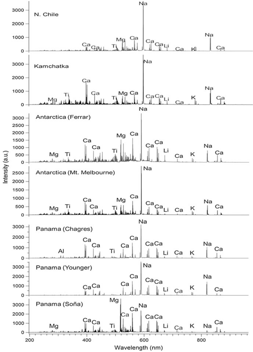
Fig. 12.11 Representative broadband LIBS spectra of volcanic samples from seven locations in the Andes (N. Chile), Kamchatka, Antarctica (Mt. Melbourne and Ferrar), and Panama (Chagres, Younger Arc, and Soña) with major emission lines labeled to show how the chemical composition varies with geographic origin [107]
