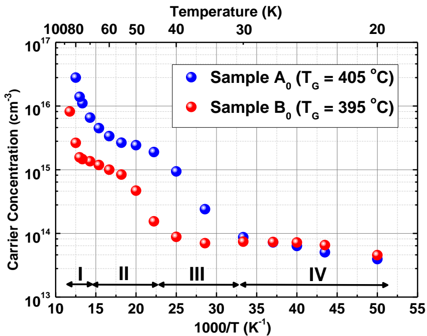
Figure 11: Comparison of the evolution of reduced carrier concentration with temperature between sample A_0 and B_0 . Sample A_0 is grown at 405^\circ\text{C} and Sample B_0 is grown at 395^\circ\text{C} .
