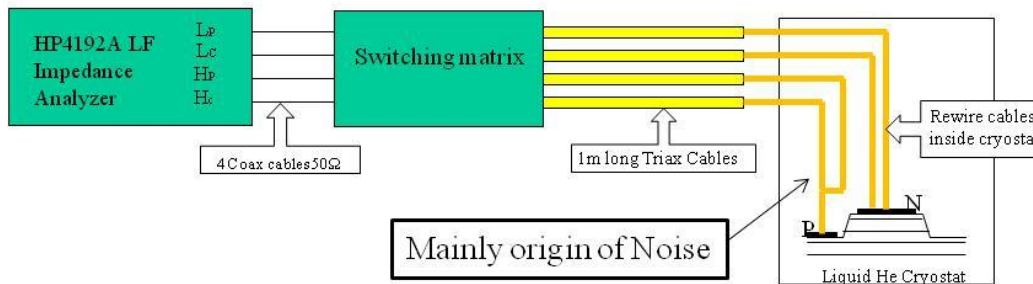
Figure 2: The schematic of the CV measurement system, including low-frequency impedance analyzer, switching matrix, liquid He cryostat and all cables.
