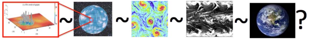
Figure 1. A visual question (left to right) asking if convective clumping in different idealized domains is similar in character ( \sim ), to each other and to the real world. Images are from Muller and Held, 2012 , AR15 , Khairoutdinov and Emanuel, 2013 , BK15 , and NASA’s Blue Marble .
