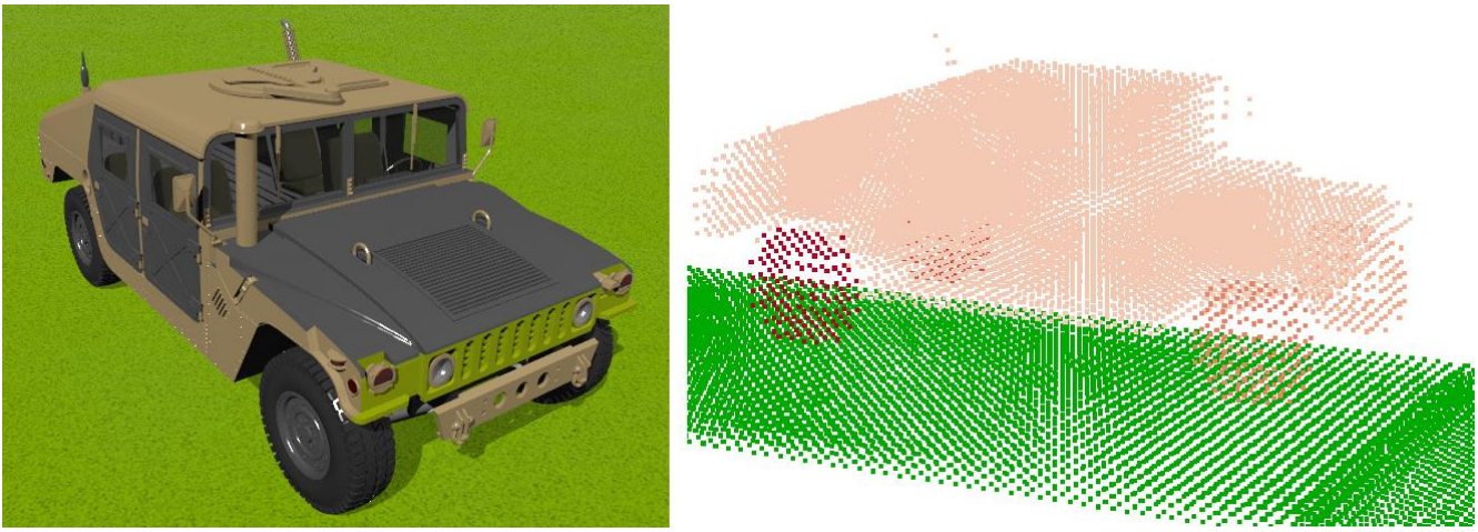
Fig. 1: The vehicle model used in a fording simulation. Any component that interacts with the fluid, such as the vehicle, tire geometries, and the solid boundaries shown in the left image, are represented as a point cloud in the fluid system. The resolution of the point cloud discretization can be changed based on the accuracy or the specific dynamics required.
