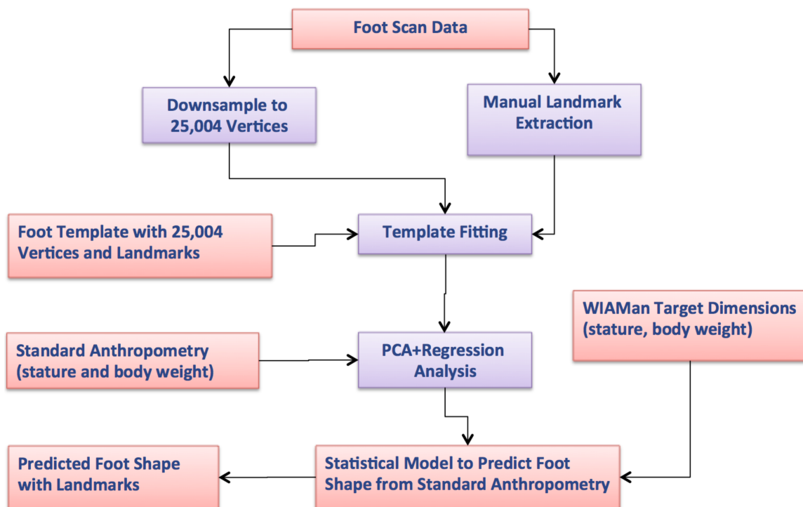
Figure 3. Data processing and analysis flowchart.
