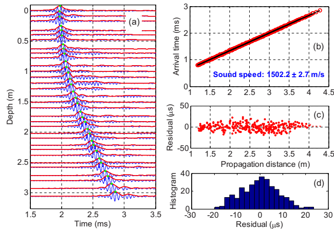
Fig. 1. (Color online) Pulse compression results at MF. (a) Waveforms received from source 10; (b) linear regression results; (c) linear regression residual scatter plot; (d) residual histogram.
