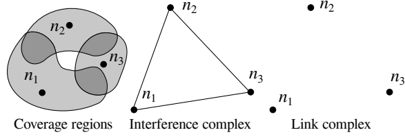
FIGURE 2. Transmitter coverage regions (left), the associated interference complex (middle), and link complex (right)
