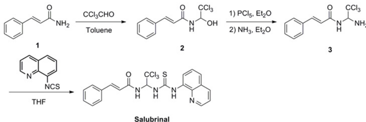
Figure 1. Synthetic route of salubrial.
