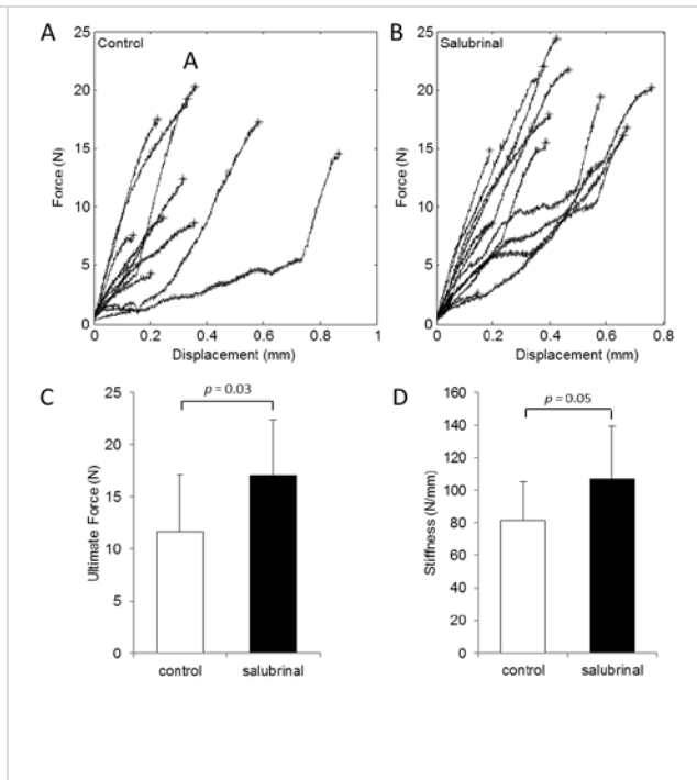
Figure 15. Mechanical strength 4 weeks after fracture induction for experiment 1. (A) Force-displacement relationship for the hydrogel control group in response to a linearly increasing displacement. The cross indicates the site of ultimate force. (B) Force-displacement relationship for the hydrogel salubrinol group. (C) Ultimate force of the hydrogel control and hydrogel salubrinol groups. (D) Stiffness of the hydrogel control and hydrogel salubrinol groups.
