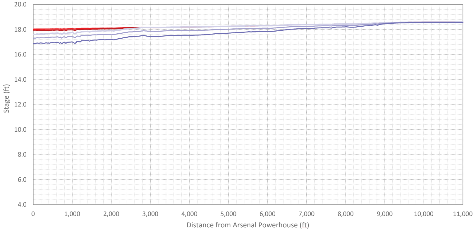
Moline Pool Stage Profile for Mississippi River Discharge of 35,000 cfs
