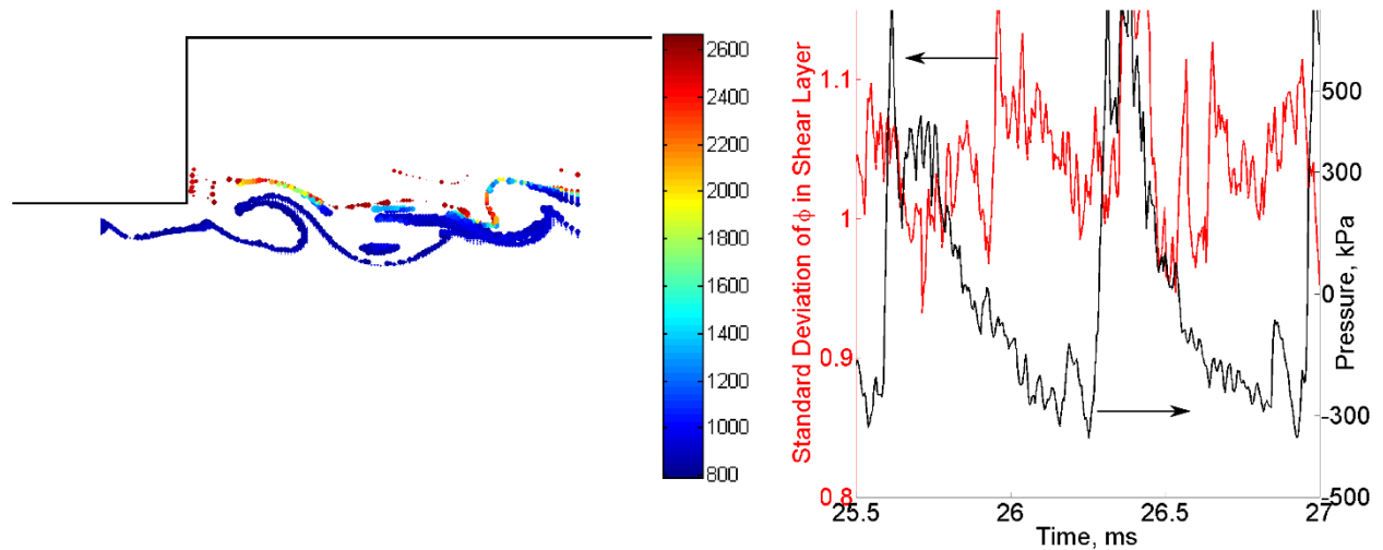
(a) Shear layer sized by equivalence ratio (0.1 - 3.5) and colored by temperature of the mixture.
