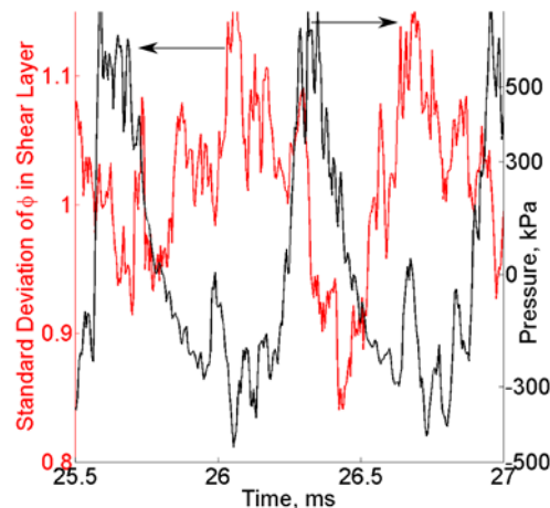
Figure 28: Unmixedness in the shear layer captured by standard deviation of the equivalence ratio.
