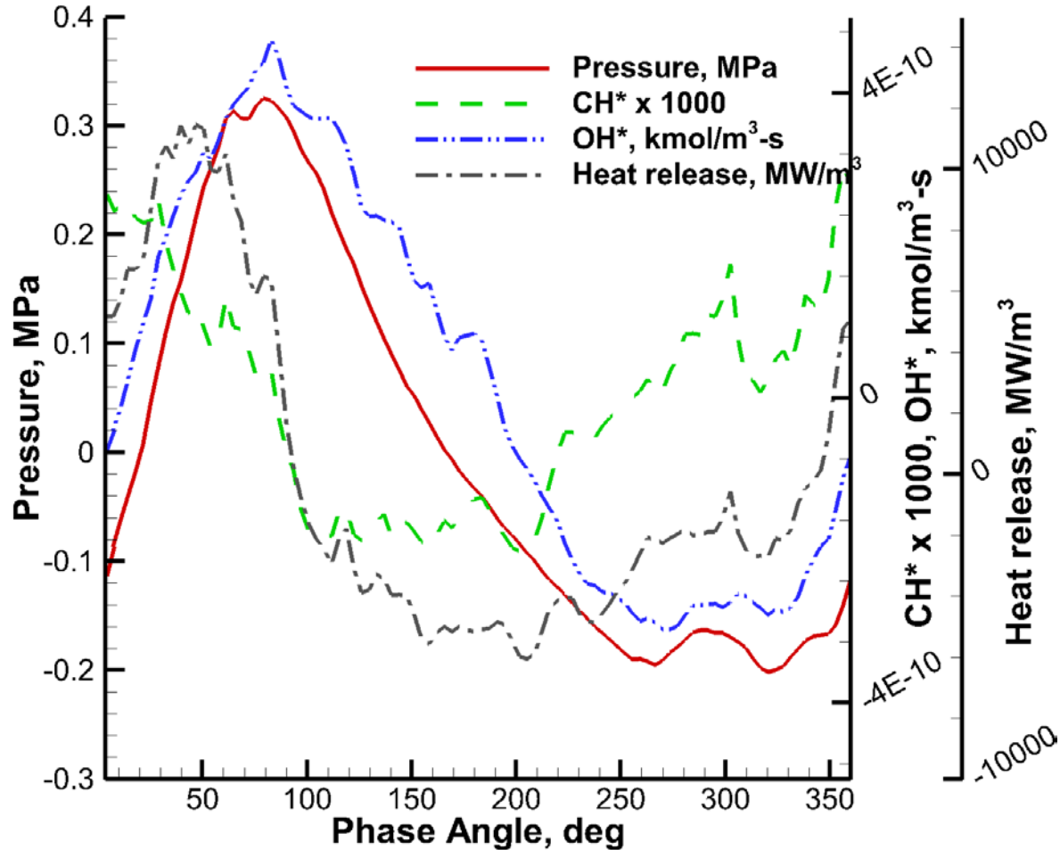
Figure 50: Phase averaged pressure heat release and radical species production rates measured from the computational model. OH^* and CH^* rates are determined by integrating throughout the probe volume with geometric weighting applied as discussed previously.
