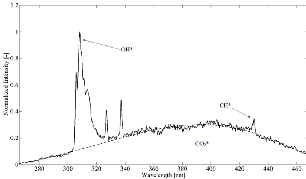
Figure 6: Average emission spectrum captured from the optic port 3 location. The most intense emissions are from \text{OH}^* and \text{CH}^* emissions near 309nm and 431nm respectively. A broadband emission from \text{CO}_2^* is observed for the full spectral width of the measurement. Two intense lines appear near 328nm and 338nm due to emission from atomic silver entrained in the oxidizer flow from the hydrogen peroxide catalyst bed.
