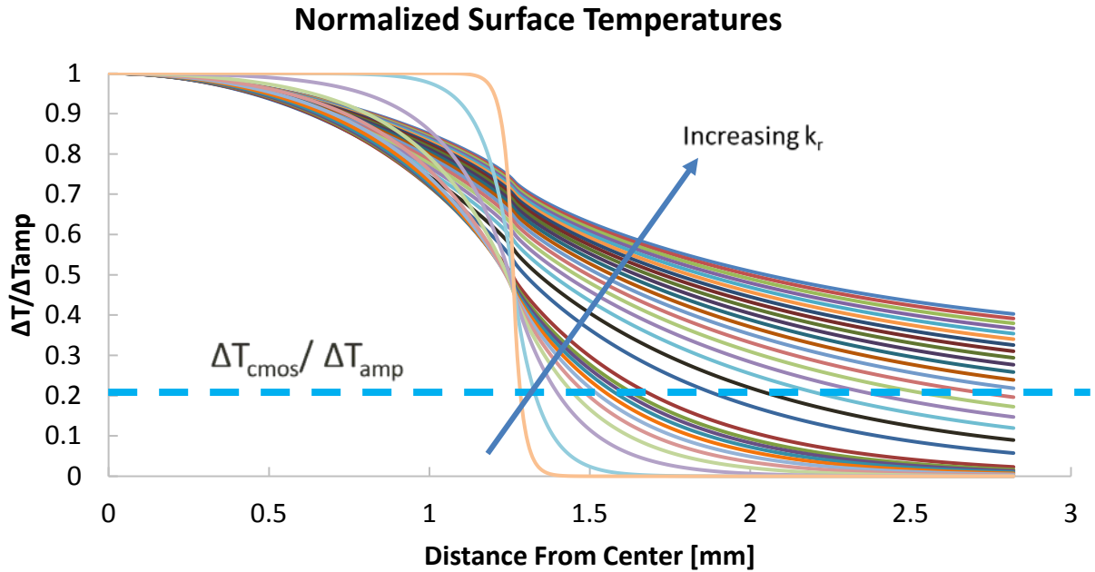
Figure 22: Interposer Surface Temperatures Normalized by Centroid Temperature As k_r increases more spreading occurs, leading to less uniform hotspot temperatures and increased device separation for strict \Delta T_{\text{cmos}}/\Delta T_{\text{amp}} ratios. However allowable amplifier dissipation increases, as according to Figure 12. The black curve corresponds to an isotropic interposer, where k_r = k_z = 150 W/m-K.
