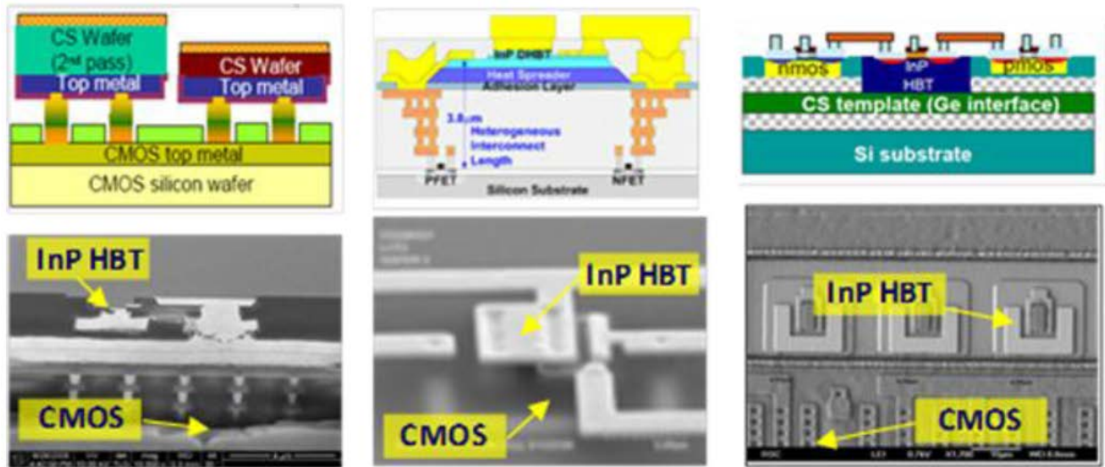
Figure 1: DAHI Integration Approaches
