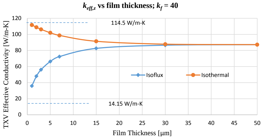
Figure 12: Evolution of k_{eff,z} of a TXV Array as an Adhered Film Increases in Thickness Film conductivity is 40 W/m-K, and substrate thickness is 200 \mu\text{m} .
