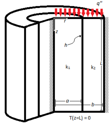
Figure 15: Schematic of Boundary Value Problem
