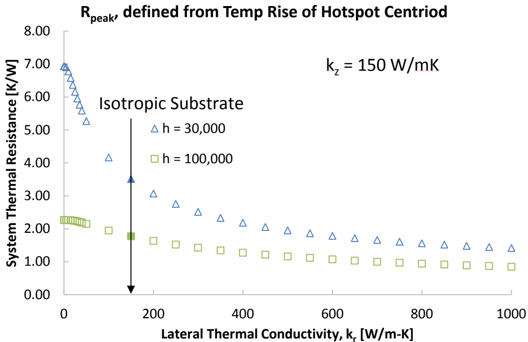
Figure 20: System Thermal Resistance, R_{peak} for Two Values of Underside Cooling Heat Transfer Coefficient
