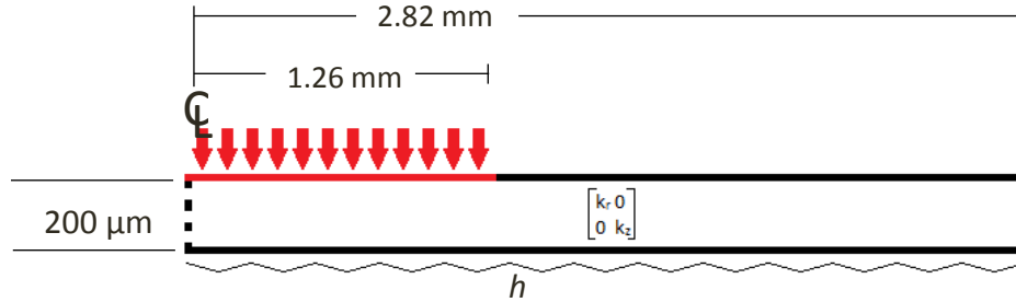
Figure 19: Schematic of Compact System Model
