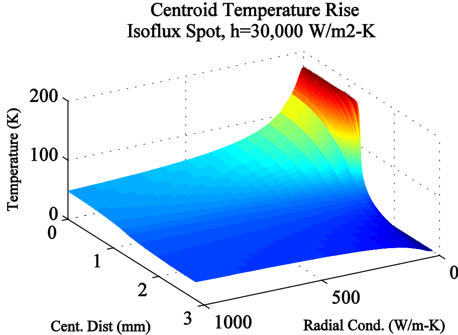
Figure 21: Raw Interposer Surface Temperature Rise for a Hotspot Flux of 500 W/cm 2 with Underside Cooling of h = 30,000 W/m 2 -K and Varying Radial Conductivity, k_r . The hotspot radius is 1.26 mm.
