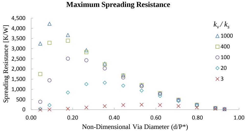
Figure 16: Maximum Cell Spreading Resistance as a Function of Via Diameter and Conductivity
