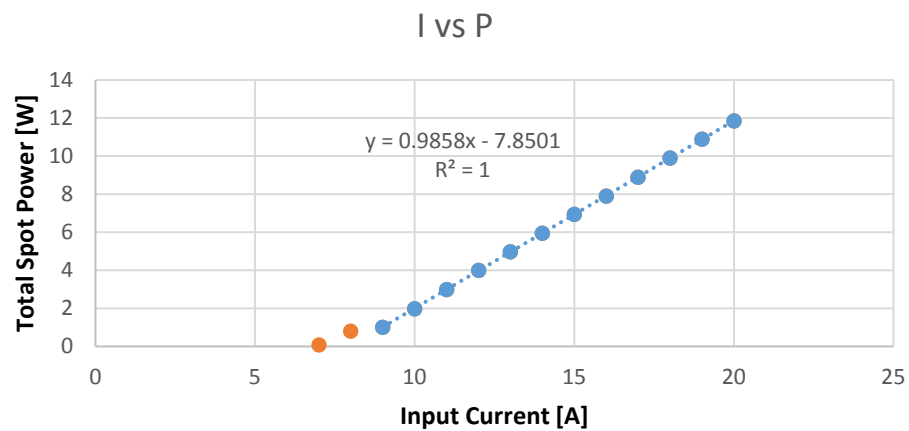
Figure 29: Laser Power Calibration Curve, Relating Spot Power to Input Current
