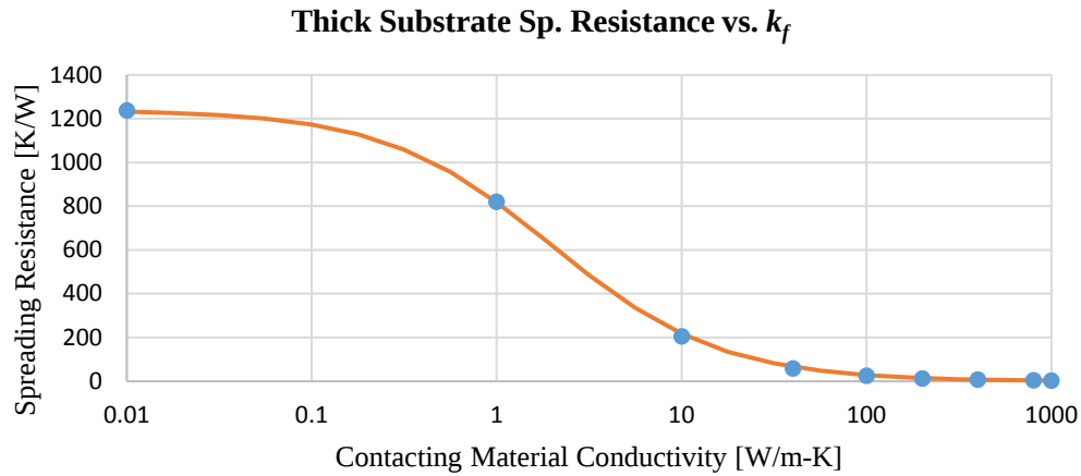
Figure 14: Spreading Resistance versus Contacting Material Conductivity Each point is obtained from FEM data in Figure 13. The line connecting the points is the correlation given by Eq. (14).
