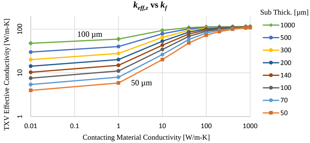
Figure 13: k_{eff,z} versus Contacting Material Thermal Conductivity for Different Substrate/Cell Thicknesses
