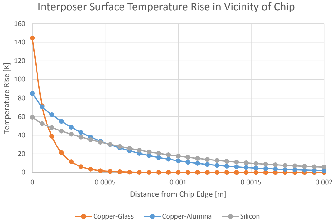
Figure 18: Interposer Surface Temperature Rise for Three Different Interposer Material Systems under the First Compact Model
