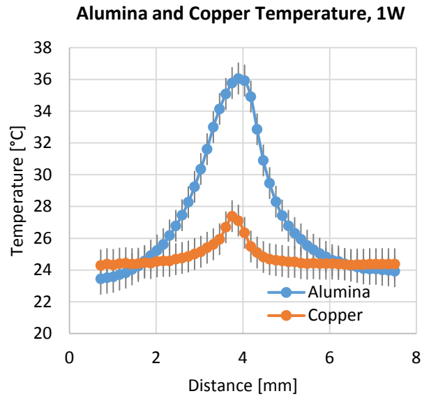
Figure 31: Reference Sample Surface Temperature Profiles through Midline from 1 W Laser Spot
