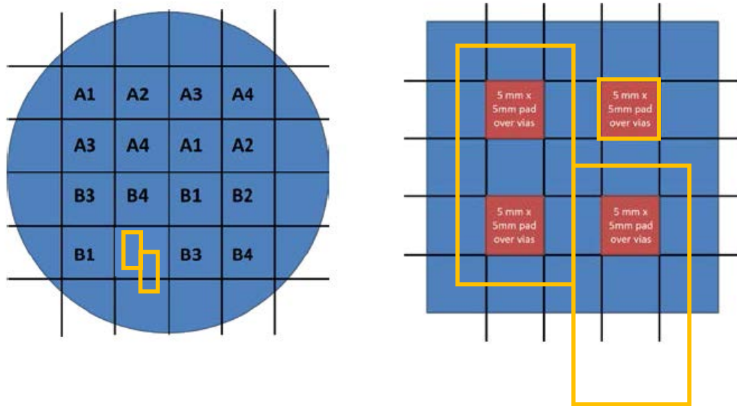
Figure 34: Sample Dicing Layout Compatible with Microgap Cooler Testing
