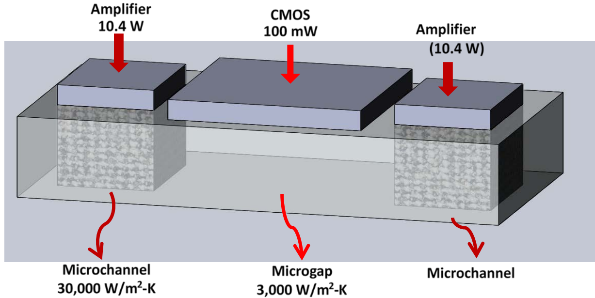
Figure 5: Rotated View of HI Case Study System Showing Input Power and Underside Cooling
