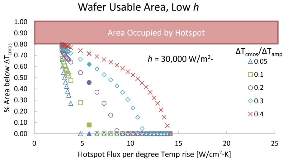
Figure 25: Usable Area vs. Normalized Hotspot Flux for h = 30,000 \text{W/m}^2\text{-K} Up and right are better. Lower cutoff ratios are more restrictive. Solid points correspond to an isotropic interposer.
