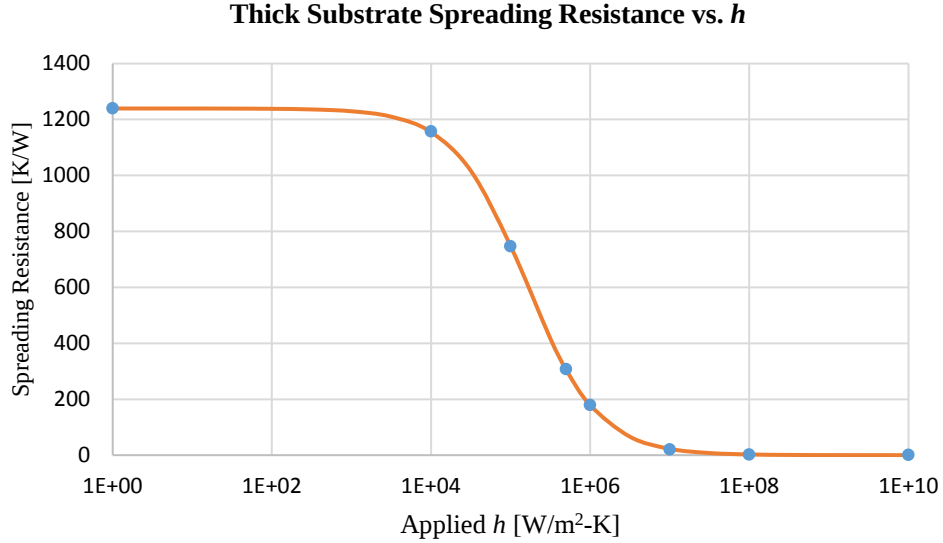
Figure 11: Spreading Resistance of Thick TXV Substrates
