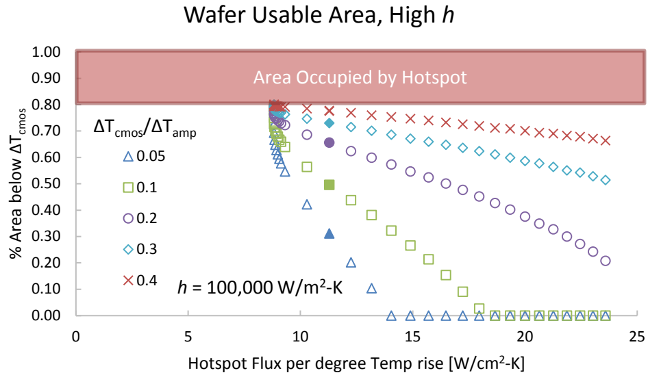
Figure 26: Usable Area vs Normalized Hotspot Flux for h = 100,000 \text{ W/m}^2\text{-K} Up and right are better. Lower cutoff ratios are more restrictive. Solid points correspond to an isotropic interposer.
