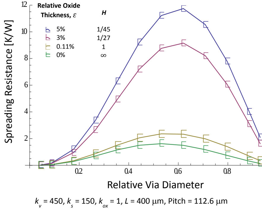
Figure 17: Spreading Resistance for a TSV-like System with Varying Interface Conductance
