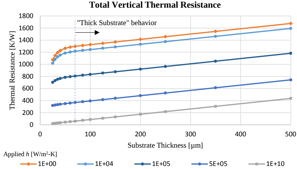
Figure 10: Via Cell Total Thermal Resistance, Calculated from k_{eff,z} Data
