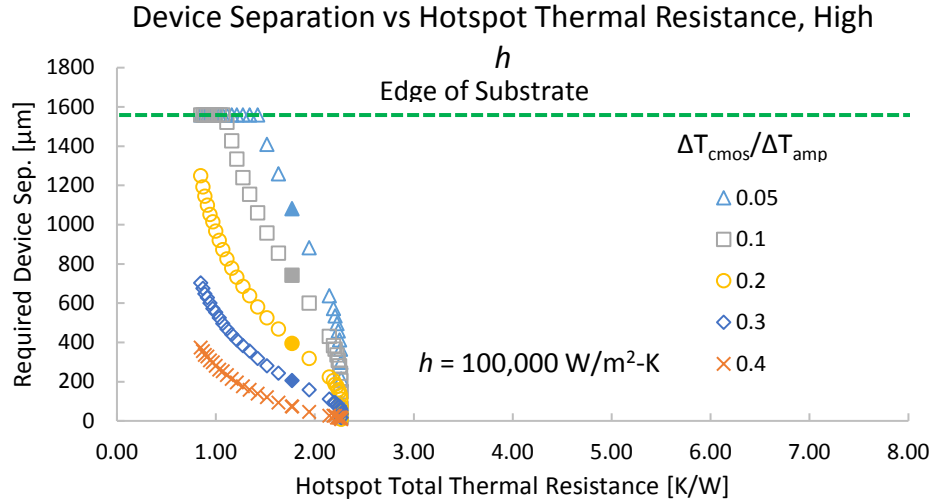
Figure 24: Device Separation vs. System Resistance Tradeoff Contours for the h = 100,000 \text{W/m}^2\text{-K} case
