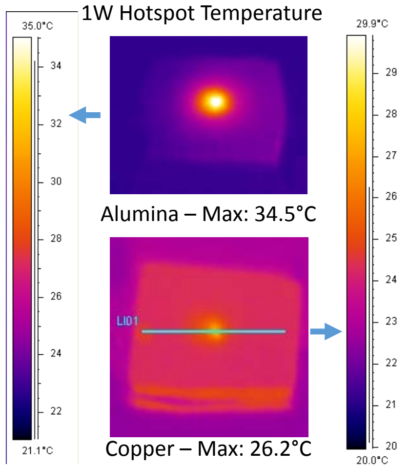
Figure 30: IR Images of Spot Heated Alumina (top) and Copper (bottom) Chiplets On the copper image is an example of a pathline for data export and analysis.
