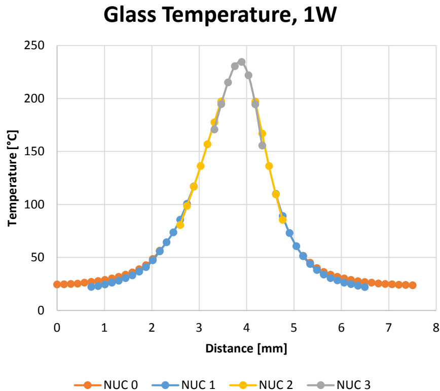
Figure 33: Glass Reference Sample Surface Temperature Profile Resulting from a 1 W Spot
