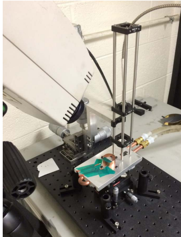
Figure 28: Experimental Setup Including infrared camera, fiber laser, and water-cooled coldplate.
