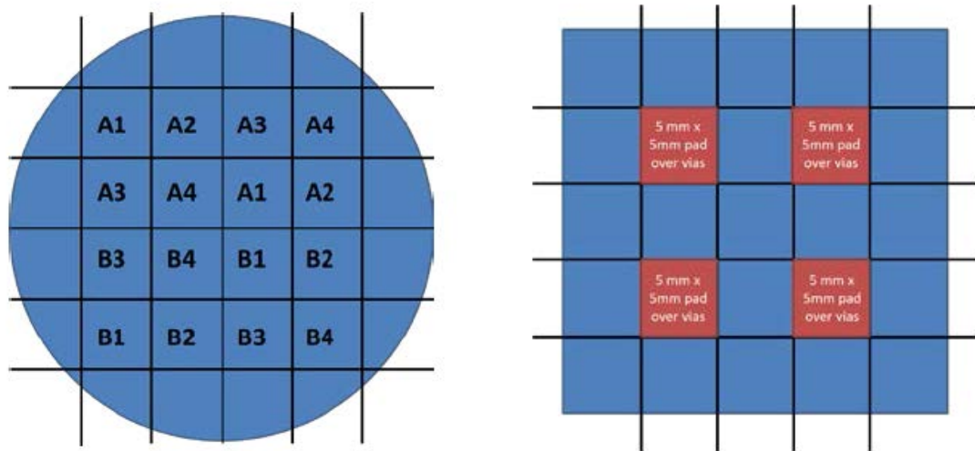
Figure 27: Glass Wafer Division into 16 Test Coupons
