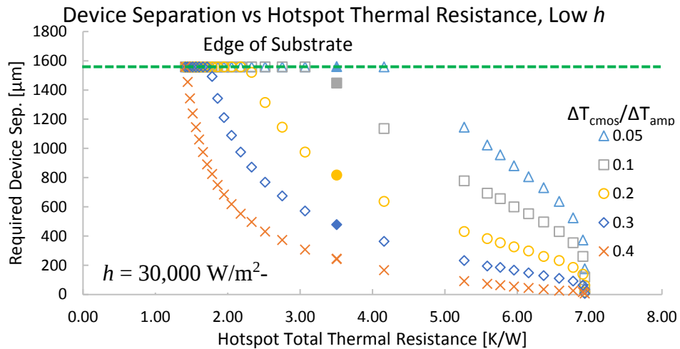
Figure 23: Device Separation vs. System Resistance Tradeoff Contours for the h = 30,000 W/m 2 -K case
