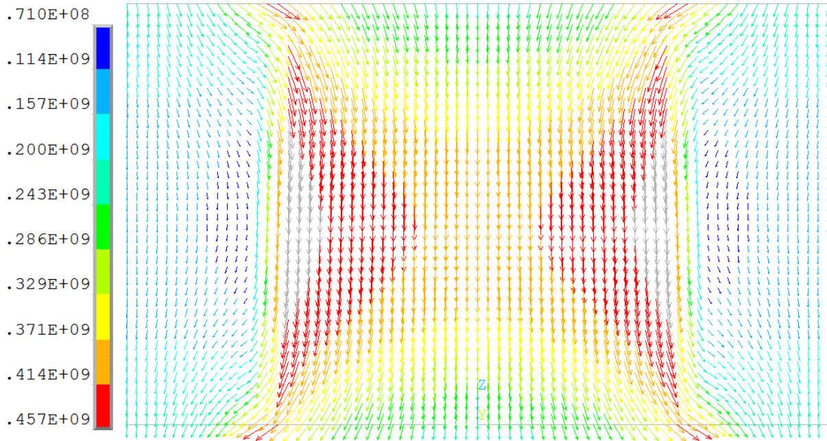
Figure 8: Heat Flux Vectors at a Vertical Cross-section of a Unit Cell
