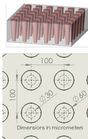
Figure 4: Array Parameters for Copper Vias
