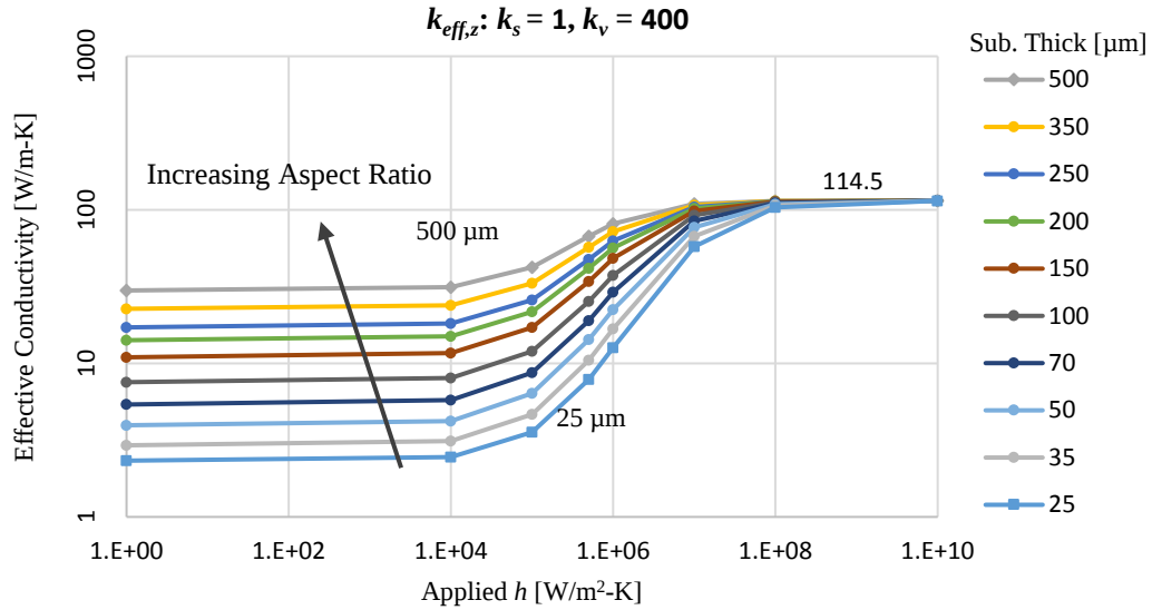
Figure 9: TXV Array k_{eff,z} as Computed by FEA
