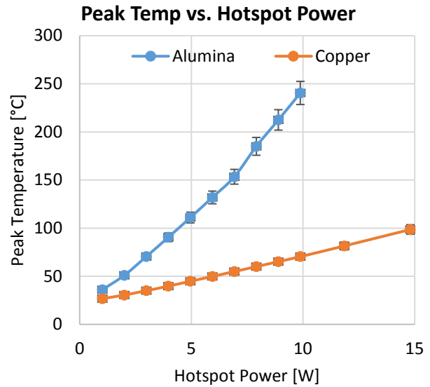
Figure 32: Peak hotspot Temperature as a Function of Laser Spot Power
