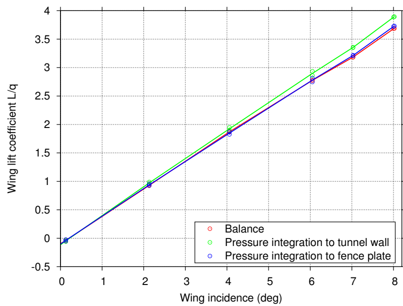
Figure 52. Comparison of wing lift measurement from balance and surface pressure integration for different incidence angles, q_{\infty} = 70 psf. (Data)
