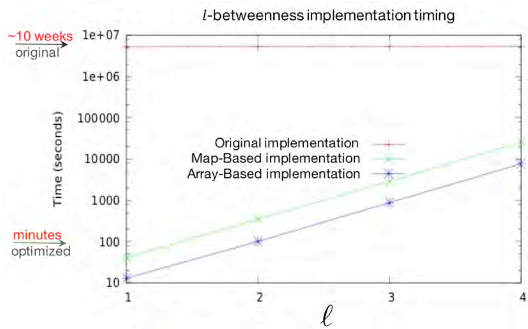
Fig 9: Orders of magnitude speed-up obtained for range-limited l -betweenness calculations using our pointer-based sparse row implementation. The test network used for this simulation was a social network inferred from cell-phone communications having 5 Million nodes and about 27 Million edges.
