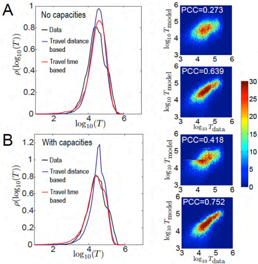
Fig 12: (A) Left panel: comparison between the densities of log(traffic) obtained from data (black line) and the model without capacity limitation based on travel distance (blue line) and travel time (red line). The heat maps are scatter plots between real traffic and model traffic values without capacity limitation. For the upper map the travel distance cost function with a range limit of 100km was used generating a PCC of 0.273. For the lower map the travel time cost function was used with a range limit of 100min and velocity classes 90-40-15mph, generating a PCC of 0.639. (B) Same as in (A) but with capacity limitation included. Here the best PCC of 0.752 was obtained configuration as in (A). The range limits here were 400km and 400min, respectively.
