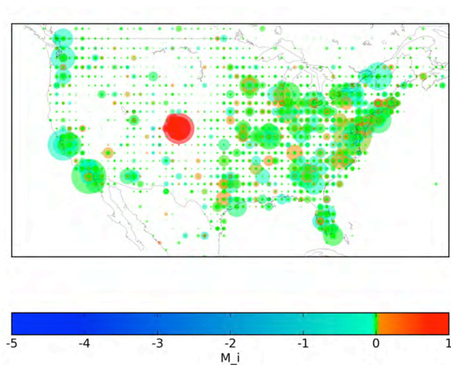
Fig 48: We show the damage assessed by a traceroute-like network exploration in the case of a large localized damage of the Internet autonomous system network in the area of Denver. It is possible to see the non-local effects (orange nodes) that ripple from the damaged area up to very distant nodes.
