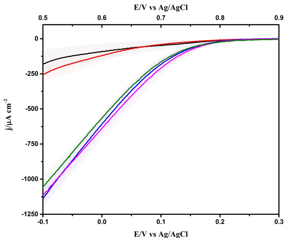
Figure 4: LSV of SZ 3 1 (SZ 3 /SWNT: black); SZ 3 2 (SZ 3 /D 2 H/SWNT: red); SZ 3 NC1 (SZ 3 /D3D 2 NCH/SWNT: magenta); SZ 3 NC2 (SZ 3 /D3D 2 HNC/SWNT: blue); and SZ 3 NC (SZ 3 /D3G/SWNT: green) composites in O 2 saturated 0.1 M potassium phosphate buffer (pH 7.5). Three individually prepared samples of each composite were tested and averaged. Standard deviation represented by the shaded areas. Potential sweep vs. Ag/AgCl was performed from 0.8 to -0.6V, scan rate=0.01V/s; and rotation rate ( \omega )= 1600 rpm. The potential was also converted to RHE using E_{\text{RHE}} = E_{\text{Ag/AgCl}} + 0.059\text{pH} E_{\text{Ag/AgCl}}^0 with E_{\text{Ag/AgCl}}^0 = 0.179 V.
