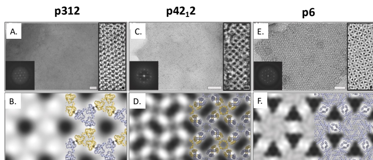
Figure 5 | Computationally designed proteins that self-assemble into unbound 2D arrays. We demonstrate one-component protein arrays with p312 (A and B), p4212 (C and D), and p6 (E and F) point symmetries. From top (A, C, E) to bottom (B, D, F) we show transmission electron micrographs of partially purified protein arrays expressed in E. coli , calculated Fourier transform electron diffraction patterns from the EM images, the calculated electron density map from Fourier transform data (inset), and superposition of the electron density map with the computer model for the designed
