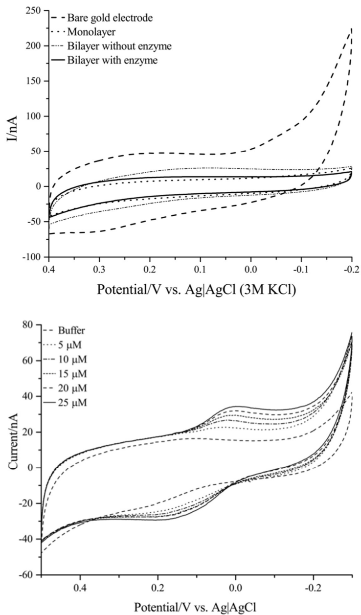
Figure 9. (Top) Cyclic voltammograms of a bare gold electrode, gold electrode with a monolayer, and gold electrode with a protein bilayer. (Bottom) Control bilayer electrode with increasing concentrations of oxidized cytochrome c. 10 mM potassium phosphate, pH 7.5, 70 mM potassium chloride. Scan rate 5 mV/s.
