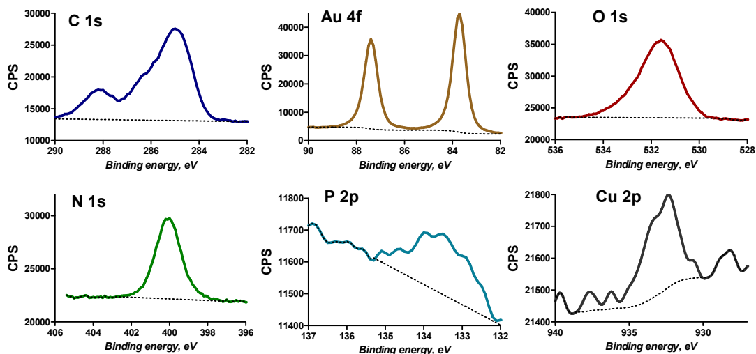
Figure 8: C 1s, Au 4f, O 1s, N 1s, P 2p and Cu 2p XPS spectra of attached SLAC-3ZNF complex onto aligned f-SWNT-arylmime modified gold surface through dsDNA scaffold.
