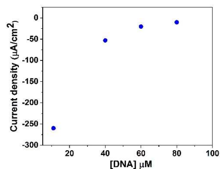
Figure S7. Effect of DNA concentration on current density (derived from LSV measurements with 10mV/s; electrode rotation rate = 1600 rpm). of SWNT/DNA/BOD composite materials in O 2 -saturated 0.1M phosphate buffer pH 7.5.
