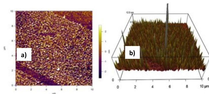
Figure 5: AFM image of Au-SWNTs sample a) 2D and b) 3D view. Size: 10 \mu m x 10 \mu m, Rate: 5 \mu m/s for 5 \mu m scan, Frequency: 0.2 Hz using super sharp silicon AFM tip.
