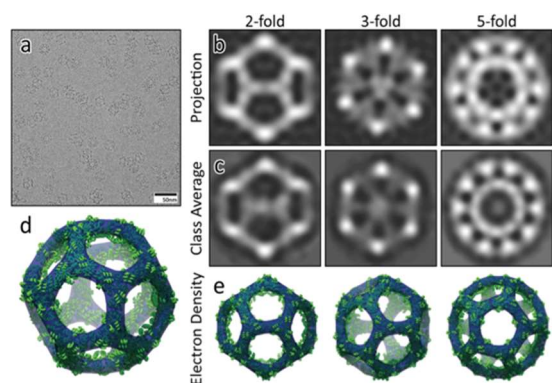
Figure 2 | Cryo-electron microscopy of a designed one-component icosahedron. a) Field of view micrographs showing monodisperse particles. b-c) Class averages along all three symmetry axes match projection images generated from the computational design model. d-e) Calculated density (blue) matches the design model (green) very well.
