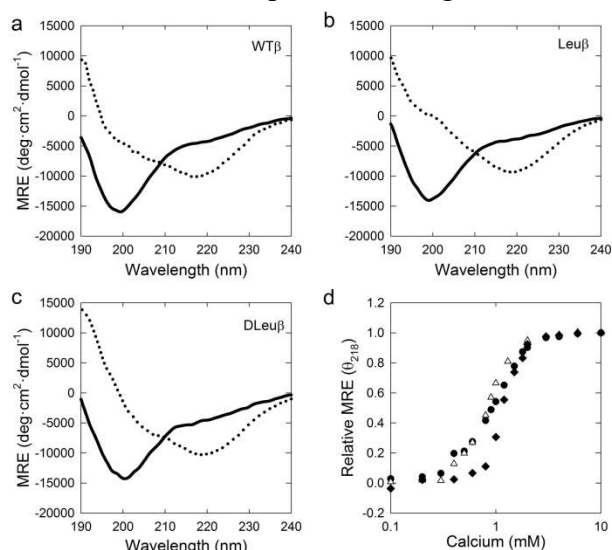
Figure 3. \beta -roll CD characterization. Mean residue ellipticity (MRE) were plotted over a range of wavelengths for WT \beta (a), Leu \beta (b), and DLeu \beta (c) in the presence (• • •) and absence (—) of 10 mM \text{CaCl}_2 . (d) Relative MRE at 218 nm for WT \beta (●), Leu \beta ( \Delta ), and DLeu \beta ( \blacklozenge ) were plotted over a range of calcium concentrations. All data were collected in triplicate in 50 mM Tris pH 7.4. Titration data were fit to the Hill equation using non-linear regression software. The calcium binding parameters are summarized in Table 1.
