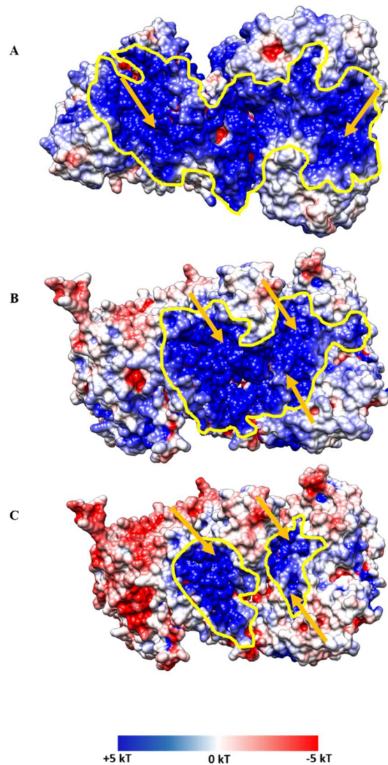
Figure 4 Simulated electrostatic channeling in WT (A), recombinant (B) and alanine-scanned (C) mMDH-CS complex. Calculation of surface ESP was done at pH 7.4. Active sites are denoted by orange arrows and electrostatic channels are highlighted by yellow edges. Negatively charged, positively charged and neutral regions are colored in red, blue and white.
