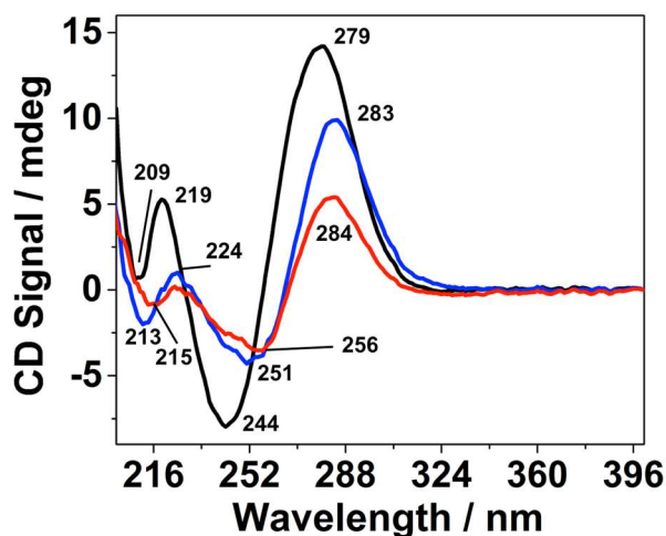
Figure 2. Secondary structural changes occur during the AuNC formation. CD spectra of solutions containing 100 \mu M DNA (black line); 150 \mu M DNA + 2250 \mu M HAuCl 4 (blue line); and the synthesized AuNC (red line).
