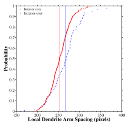
Figure 4. The cumulative distribution plot of the primary dendrite arm spacings for both interior and exterior dendrite cores in Figure 2. The solid lines represent the mean dendrite arm spacings, which can be compared to the bulk measurement of 248.4 \mu\text{m} .
