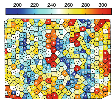
(a) Primary dendrite arm spacing ( \mu\text{m} )
