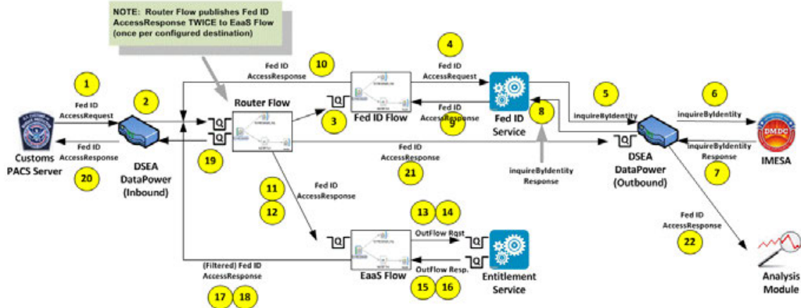
FIGURE 5. DSEA TD #2 ACCESS REQUEST USE CASE.
