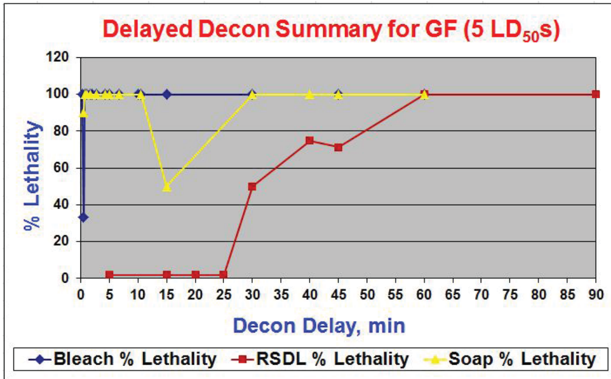
Figure 4. Graph of percent lethality when 0.5% bleach, RSDL, and 1% soapy water decontamination was delayed following challenge by 38.8 mg/kg (5 LD 50 s) of neat GF. LT 50 (50% lethality time with 95% CI) values for bleach and RSDL were 0.234* (0.065, 0.845) and 34.6 (28.3, 41.7) minutes, respectively. *The LT 50 for bleach was estimated using the less conservative delta method instead of the standard, very conservative Fieller's method. The LT 50 value for 1% soapy water was estimated to be < 0.5 minutes by using a sequential limit test and observing 9 out of 10 deaths at a delay time of 0.5 minutes. The dose-response curve slopes (95% CI) for 0.5% bleach and RSDL were 2.04 (-0.270, 4.34) and 8.28 (3.07, 13.5), respectively.
