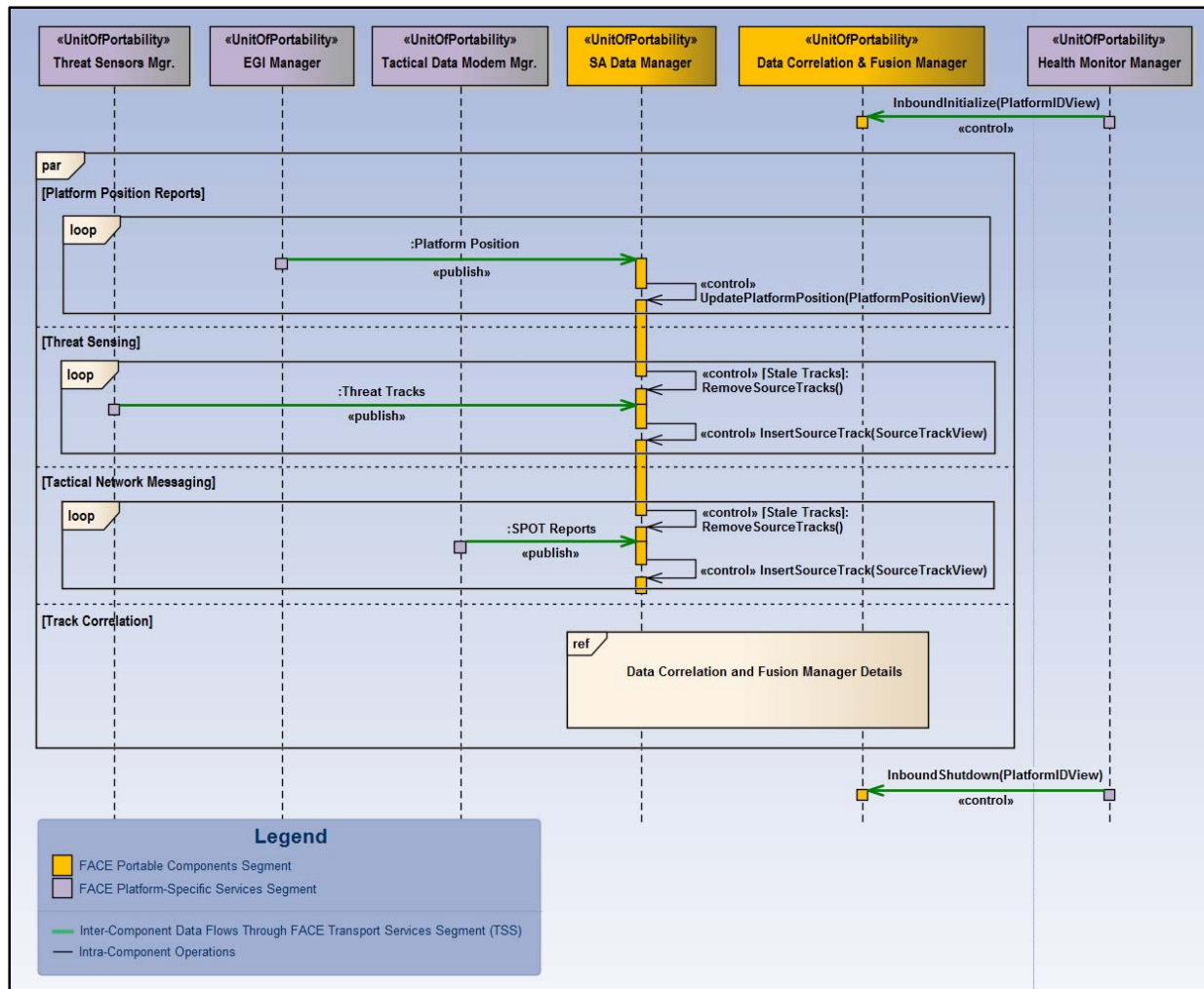
Figure A-1. Component Level Interactions (Systems View)
