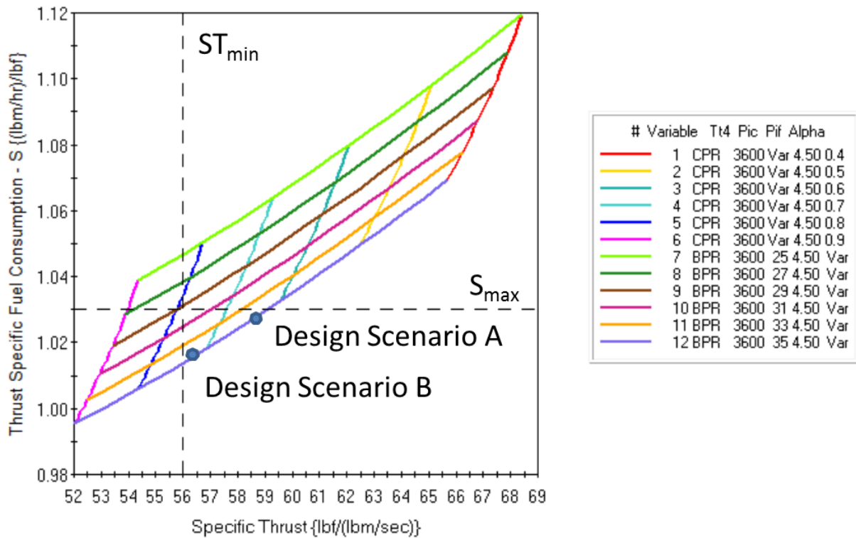
Figure 5. Parametric cycle analysis carpet plot for supercruising (M=1.5, h=36,000 ft) with Level of Technology 4 inputs to include Tt4=3600 R with 18% coolant flow bled from the high pressure compressor and injected evenly into the turbine nozzle guide vane and first stage rotor. Cycle design choice for Scenario A – alpha (bypass ratio) = 0.64, OPR = 35, Pi f = 4.5; for Scenario B – alpha (bypass ratio) = 0.72, OPR = 35, Pi f = 4.5.
