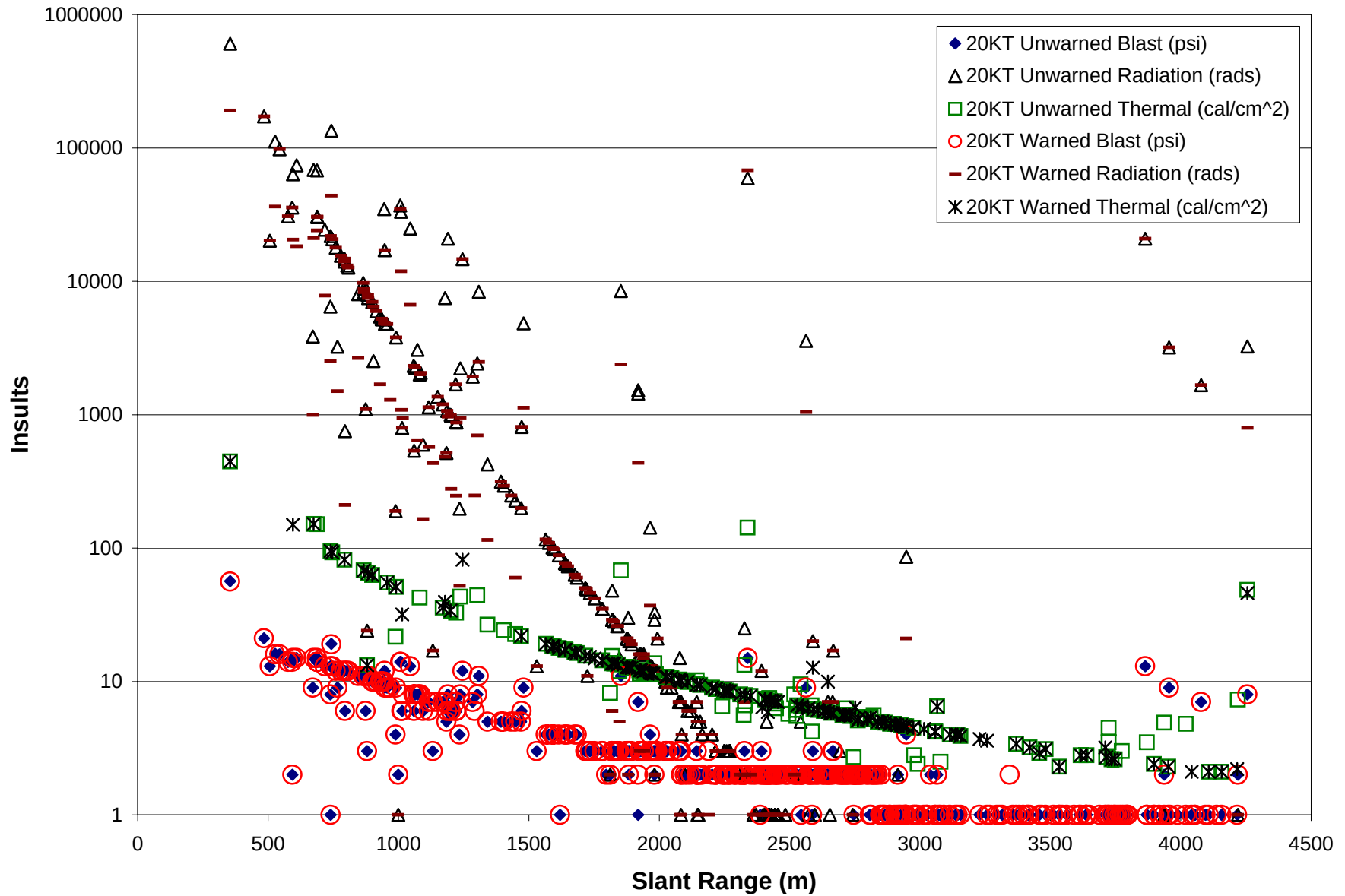
Fig. F2-2 Blast, Radiation, and Thermal Insults- 20KT Support Brigade
