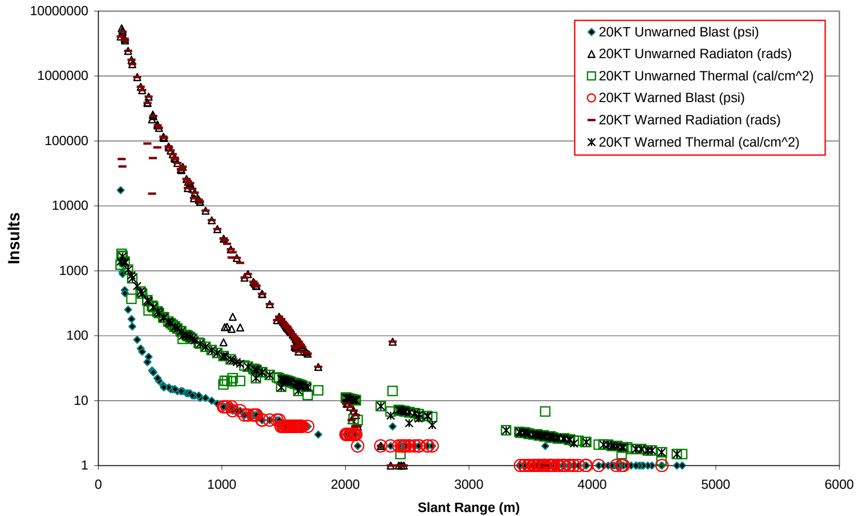
Fig. B2-2 Blast, Radiation, and Thermal Insults- 20KT Heavy Brigade, Brigade Support Area Task Force, Movement to Contact
