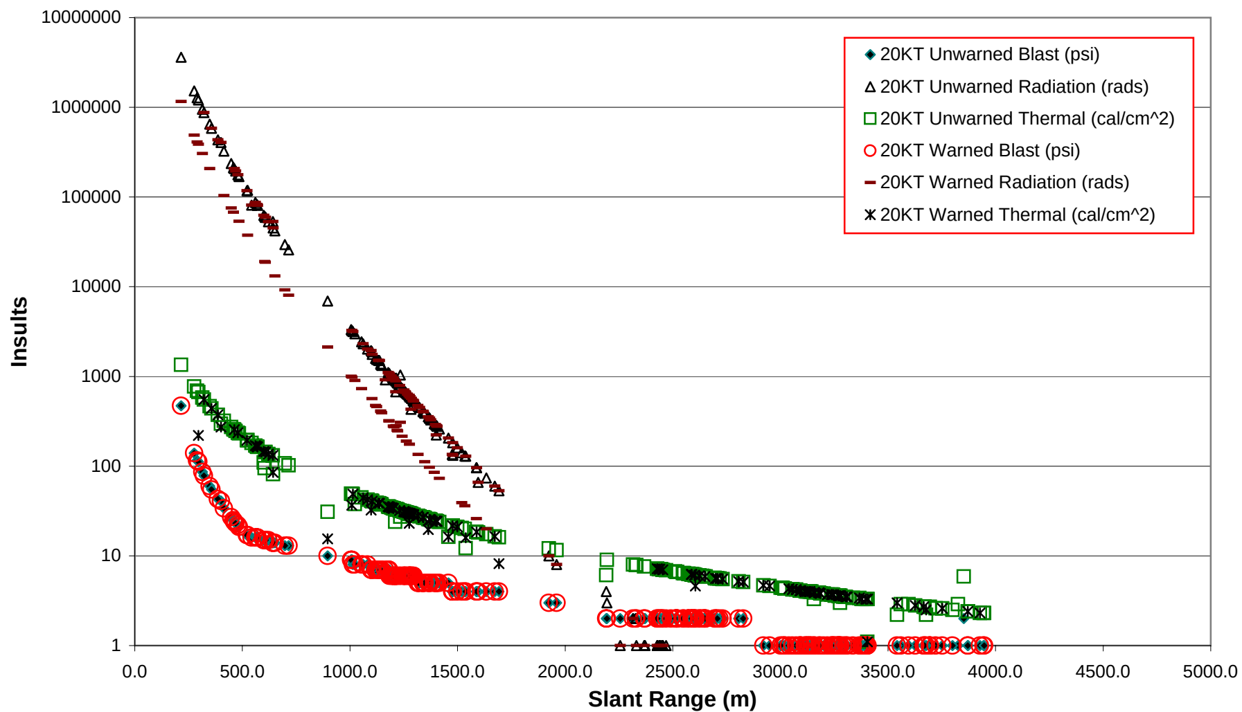
Fig. E2-2 Blast, Radiation, and Thermal Insults- 20KT Heavy Brigade, Brigade Support Area Task Force, Offense and Defense
