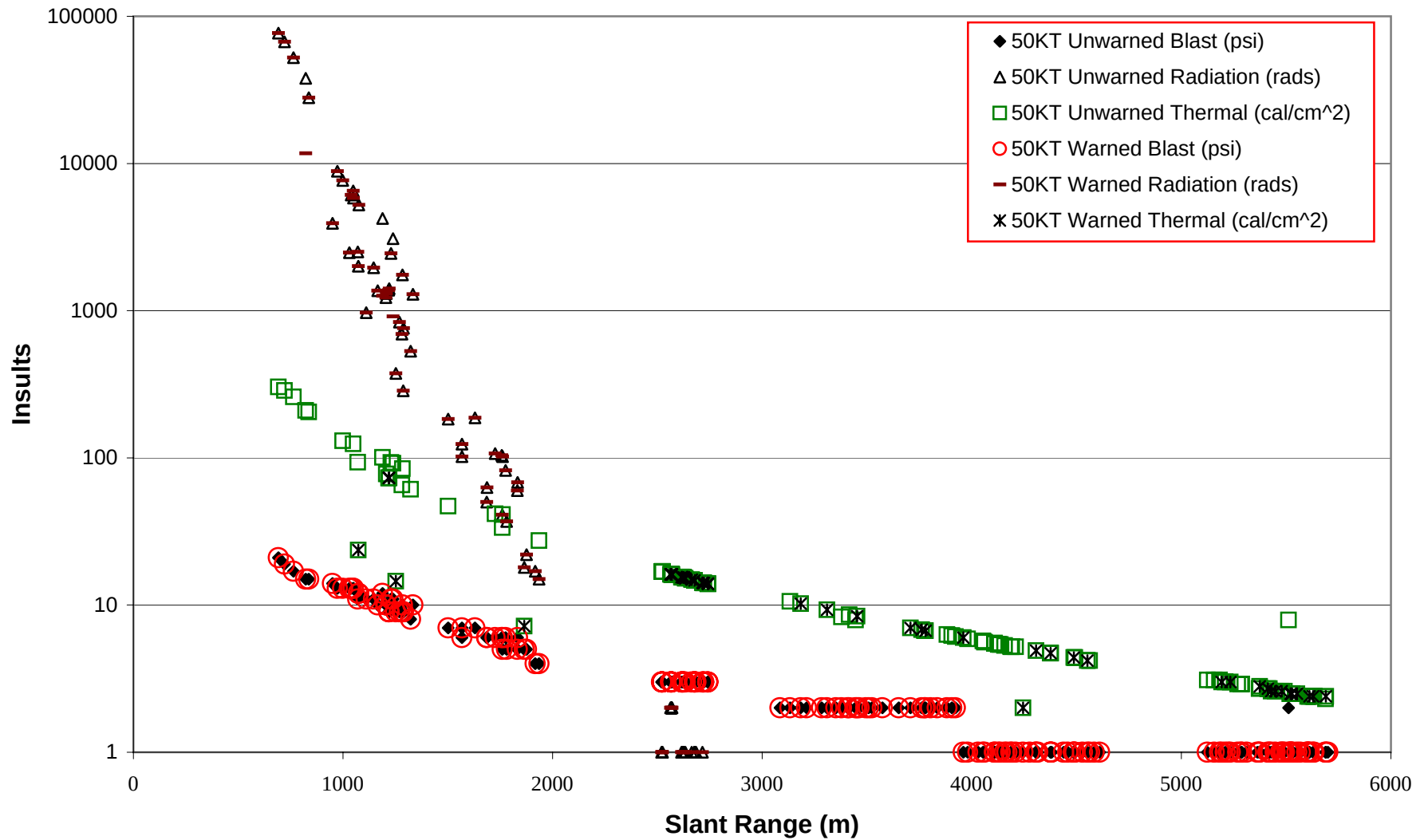
Fig. D2-3 Blast, Radiation, and Thermal Insults- 50KT Heavy Brigade, Forward Maneuver Battalion, Defense
