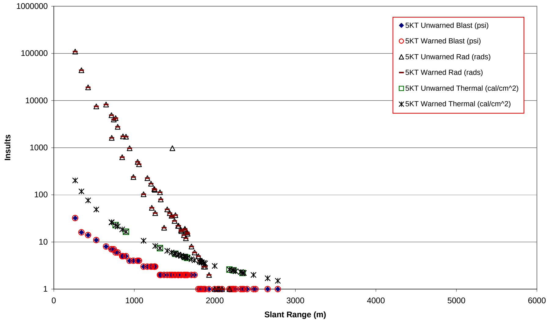
Fig. C2-1 Blast, Radiation, and Thermal Insults- 5KT Heavy Brigade, Forward Maneuver Battalion, Offense
