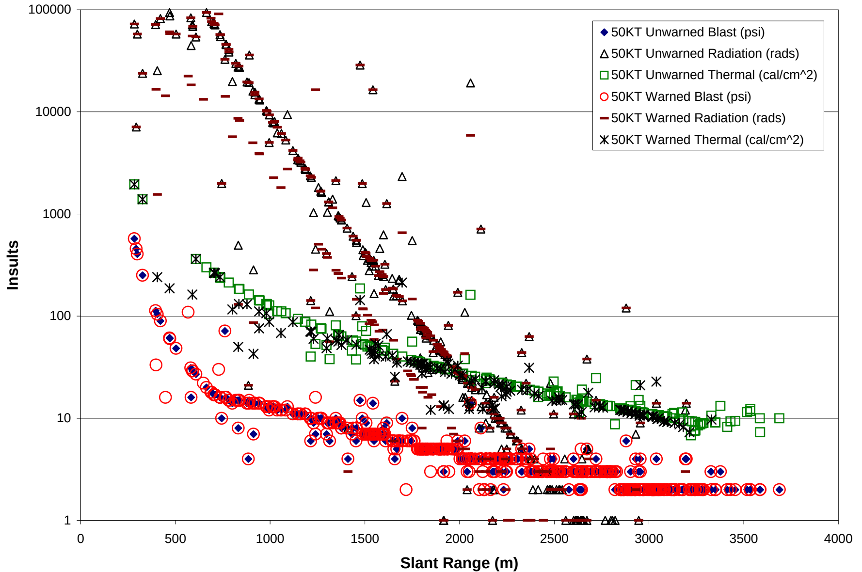
Fig. F2-3 Blast, Radiation, and Thermal Insults- 50KT Support Brigade
