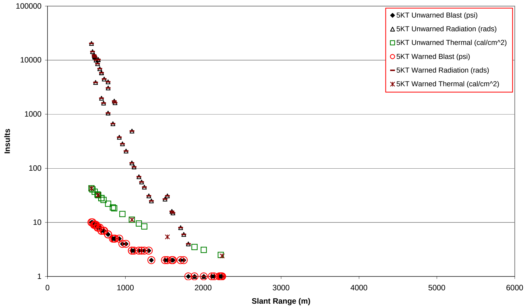
Fig. A2-1 Blast, Radiation, and Thermal Insults- 5KT Heavy Brigade, Forward Maneuver Battalion, Movement to Contact
