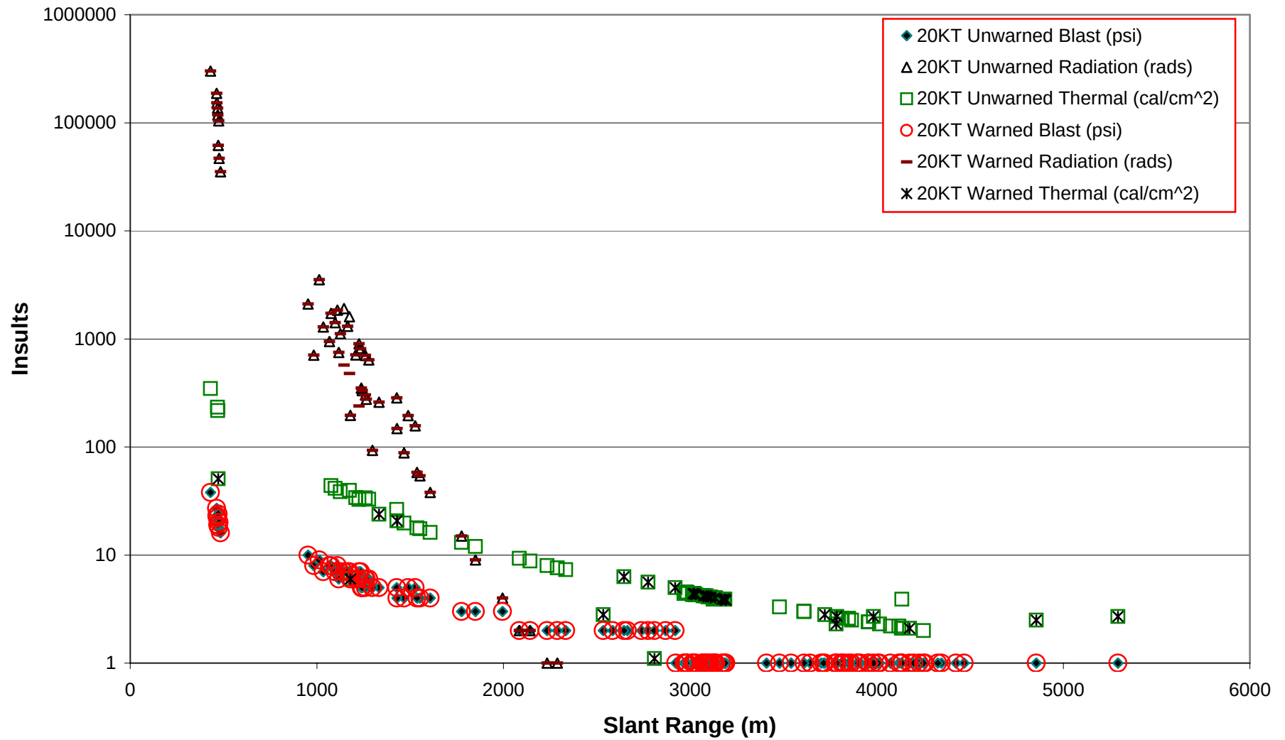
Fig. D2-2 Blast, Radiation, and Thermal Insults- 20KT Heavy Brigade, Forward Maneuver Battalion, Defense
