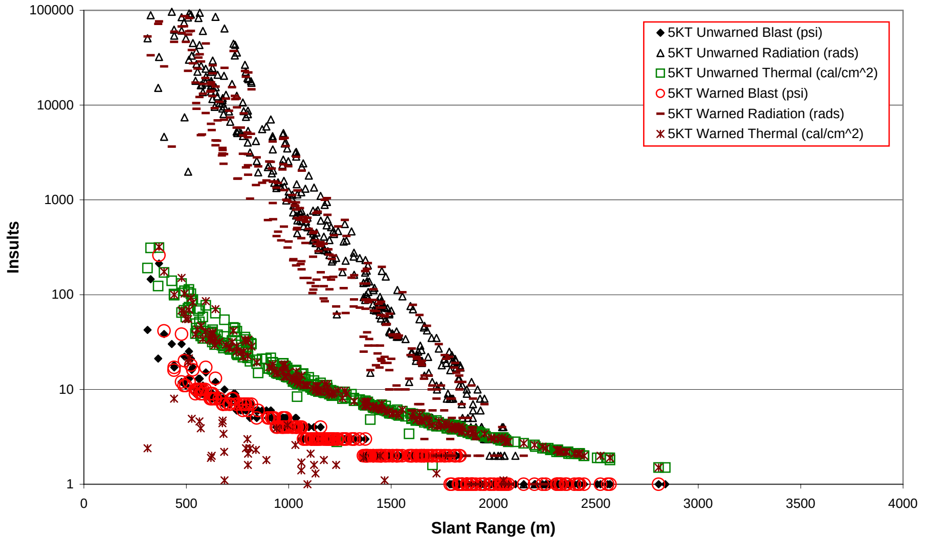
Fig. G2-1 Blast, Radiation, and Thermal Insults- 5KT Light Infantry Brigade, Defense
