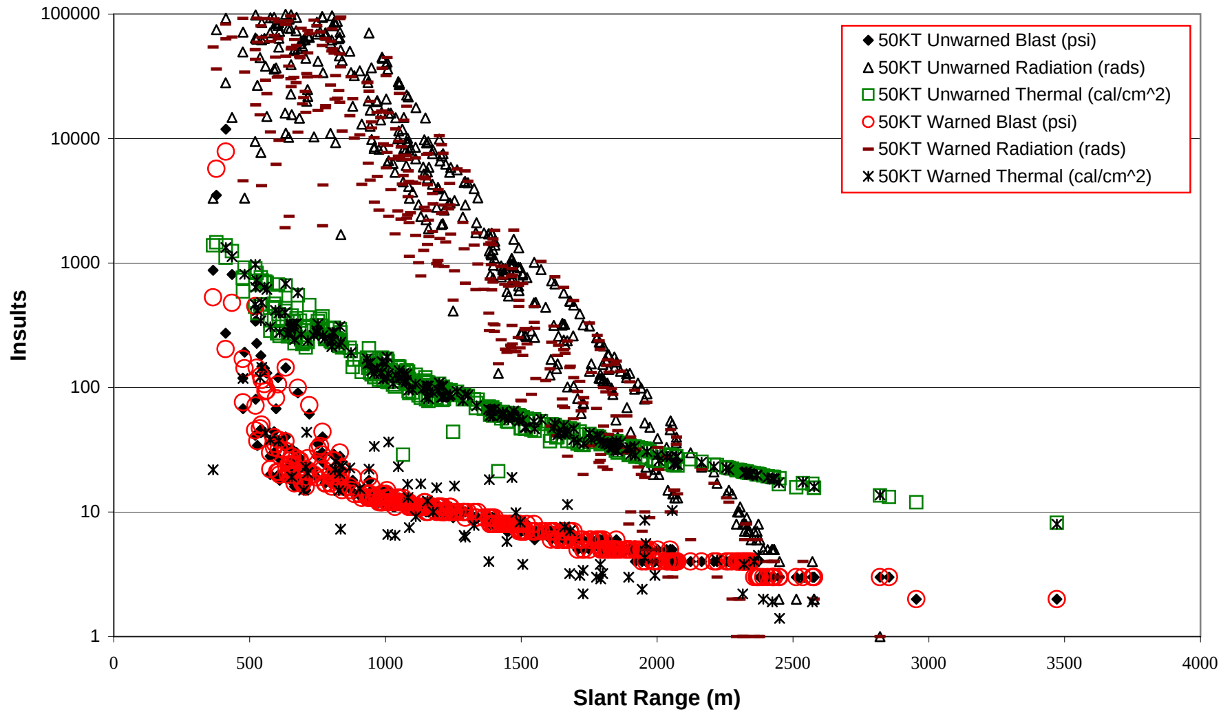
Fig. G2-3 Blast, Radiation, and Thermal Insults- 50KT Light Infantry Brigade, Defense
