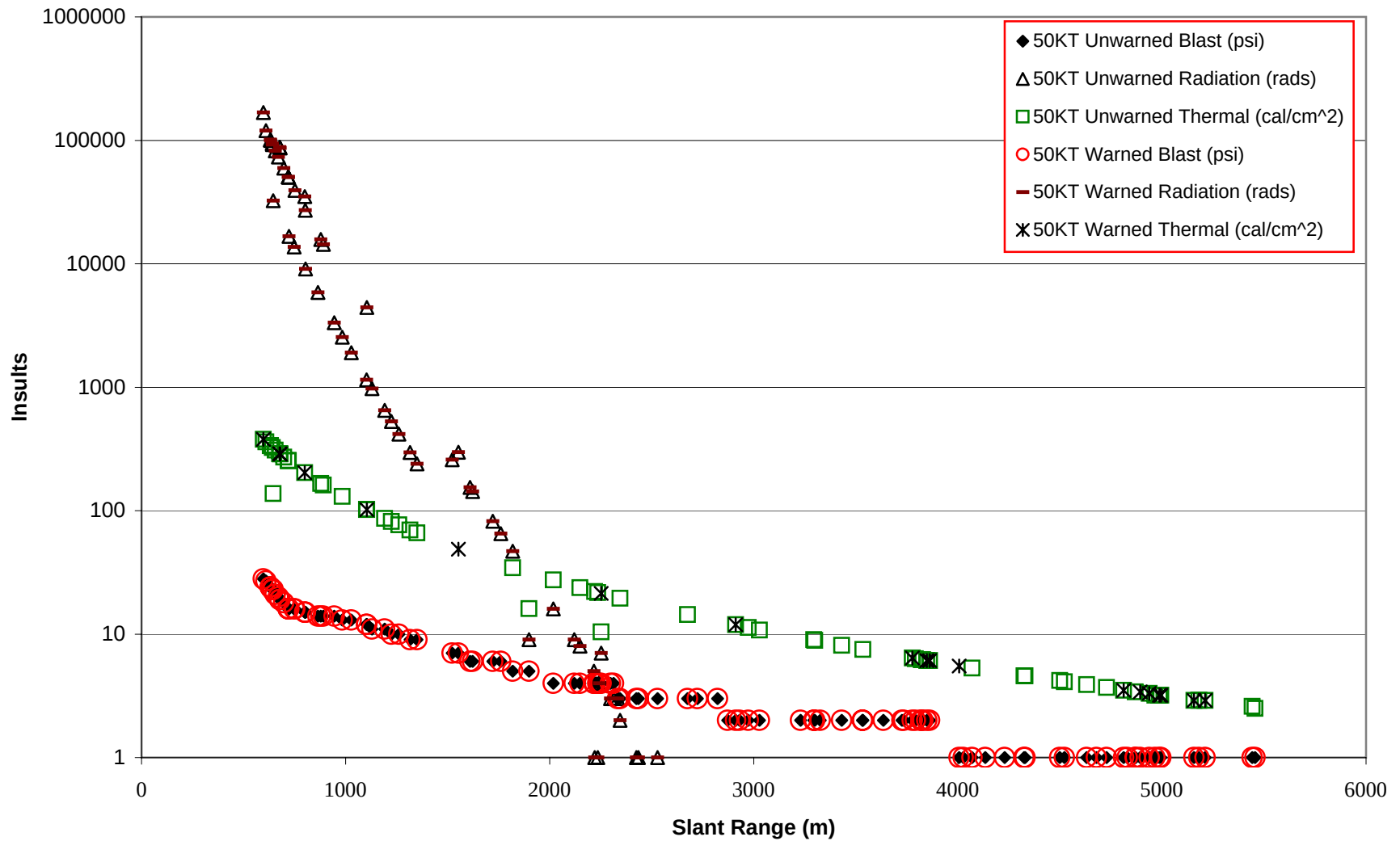
Fig. A2-3 Blast, Radiation, and Thermal Insults- 50KT Heavy Brigade, Foward Maneuver Battalion, Movement to Contact
