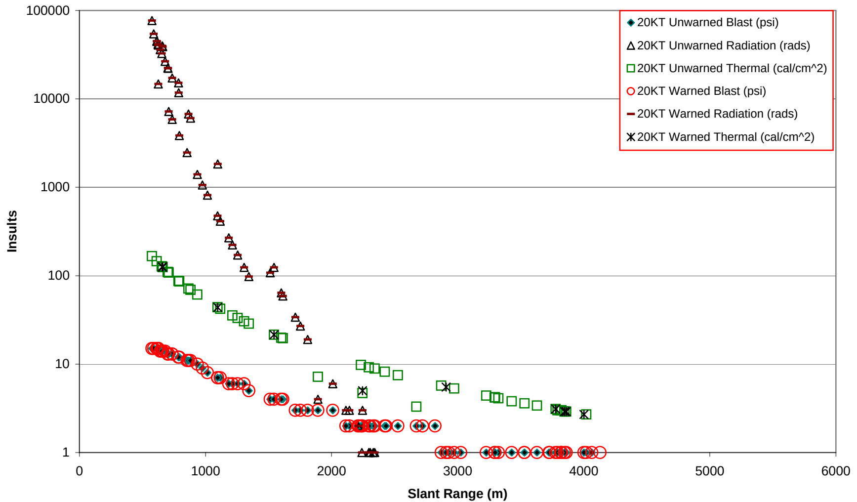
Fig. A2-2 Blast, Radiation, and Thermal Insults- 20KT Heavy Brigade, Forward Maneuver Battalion, Movement to Contact
