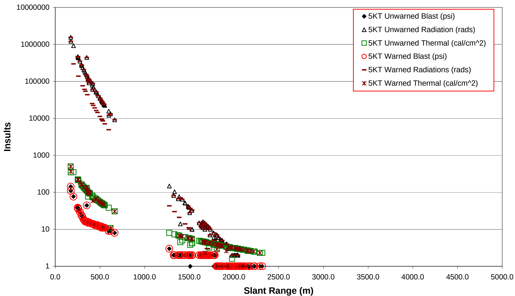
Fig. E2-1 Blast, Radiation, and Thermal Insults- 5KT Heavy Brigade, Brigade Support Area Task Force, Offense and Defense
