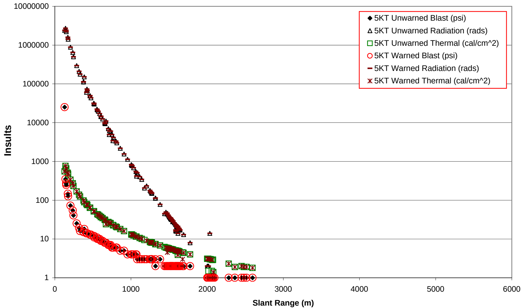
Fig. B2-1 Blast, Radiation, and Thermal Insults- 5KT Heavy Brigade, Brigade Support Area Task Force, Movement to Contact
