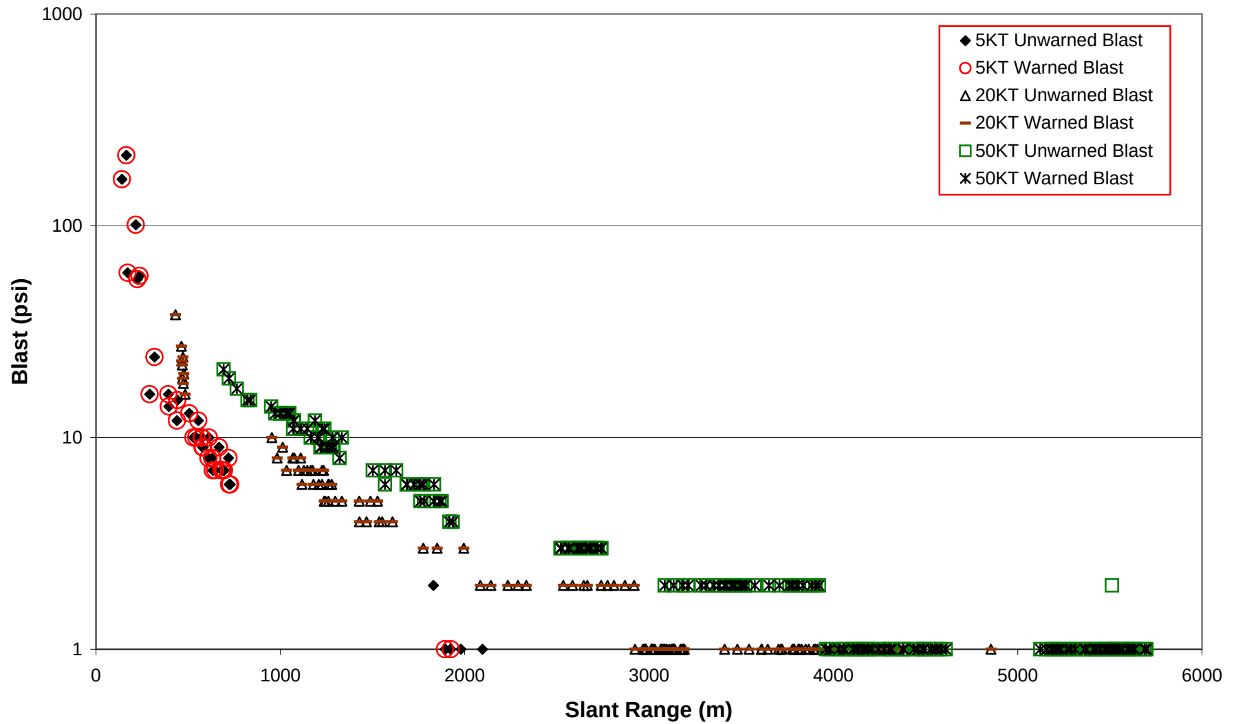
Fig. D3-1 Blast Insults Heavy Brigade, Forward Maneuver Battalion, Defense
