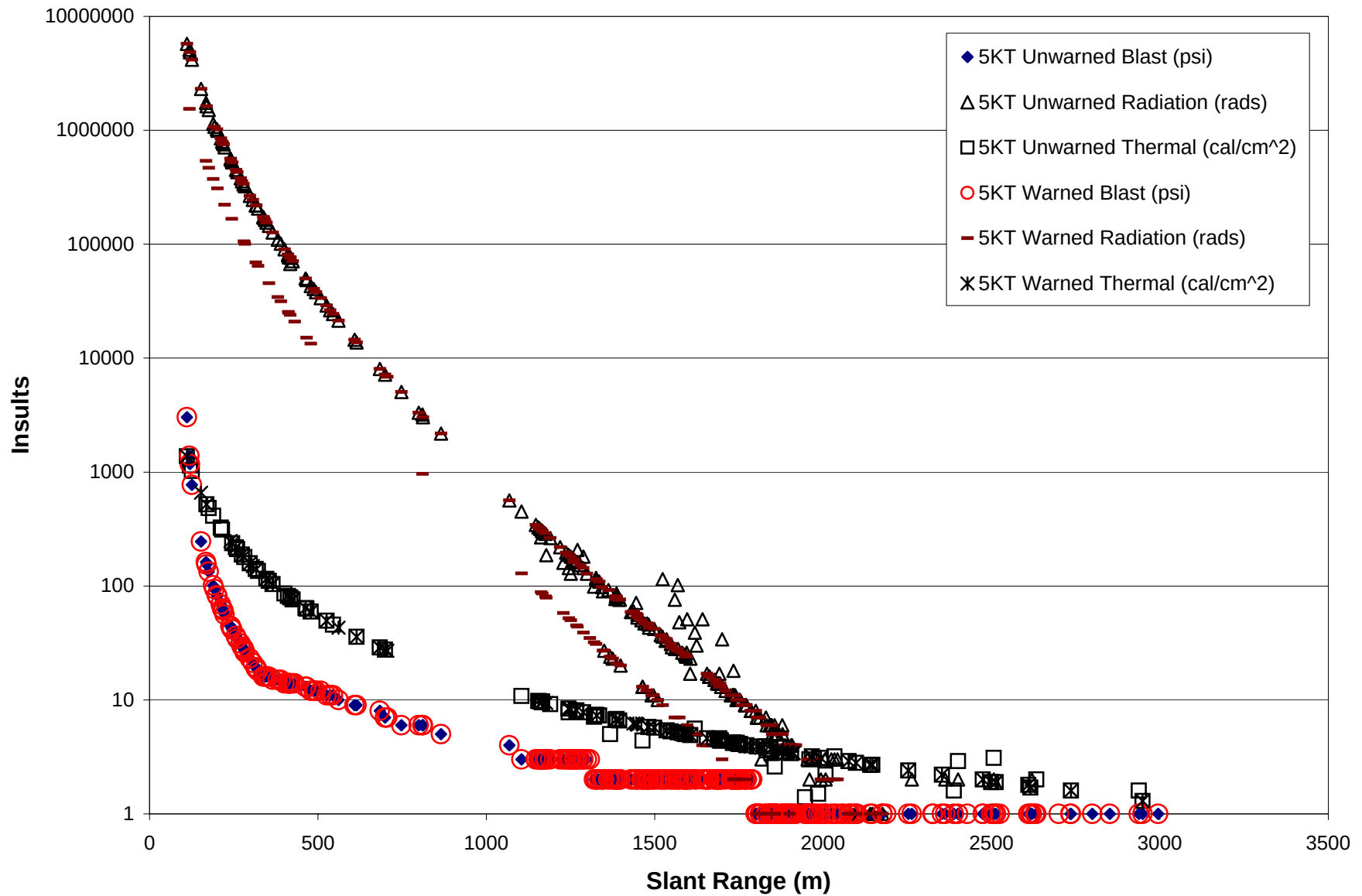
Fig. F2-1 Blast, Radiation, and Thermal Insults- 5KT Support Brigade
