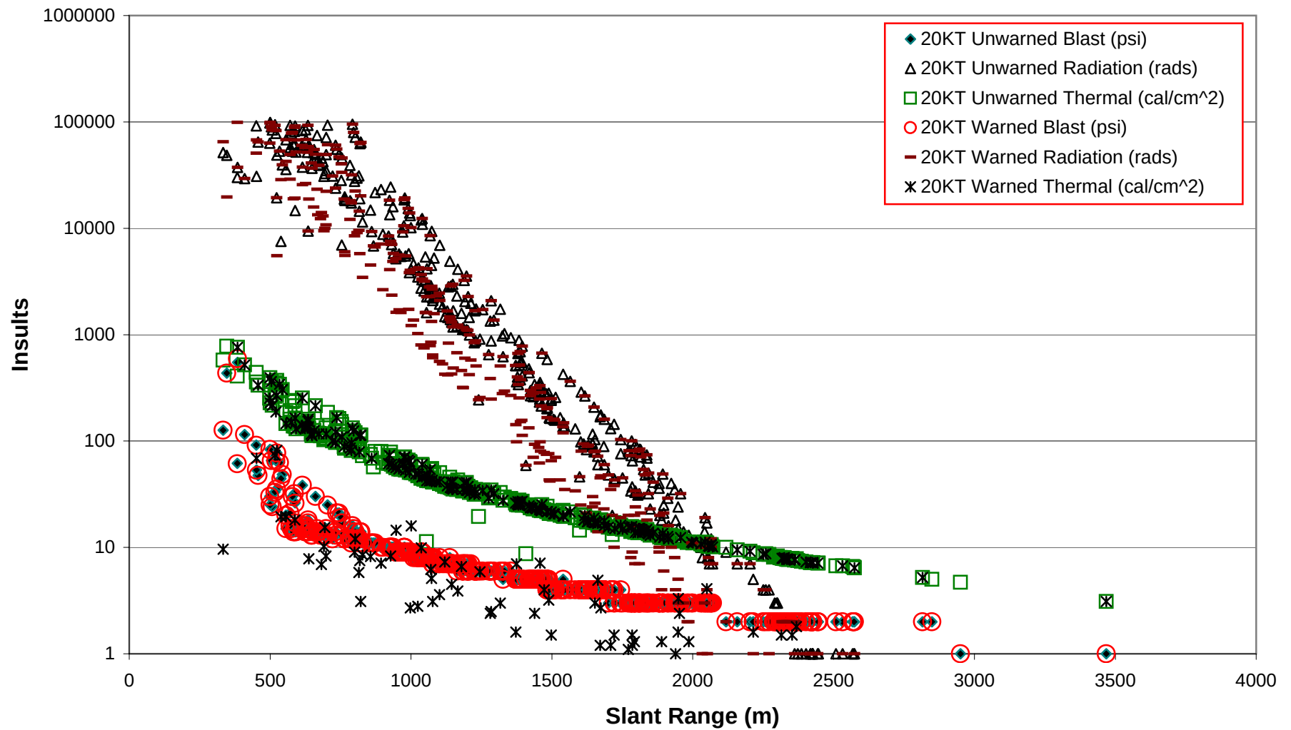
Fig. G2-2 Blast, Radiation, and Thermal Insults- 20KT Light Infantry Brigade, Defense
