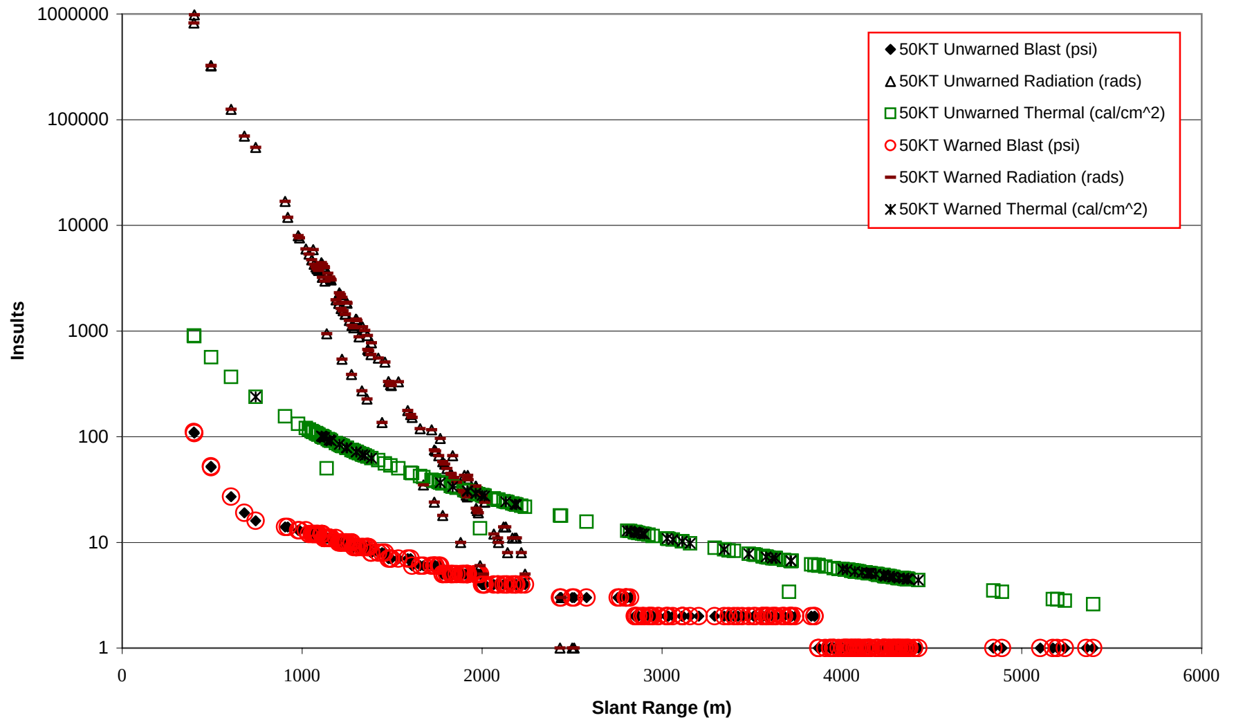
Fig. C2-3 Blast, Radiation, and Thermal Insults- 50KT Heavy Brigade, Forward Maneuver Battalion, Offense
