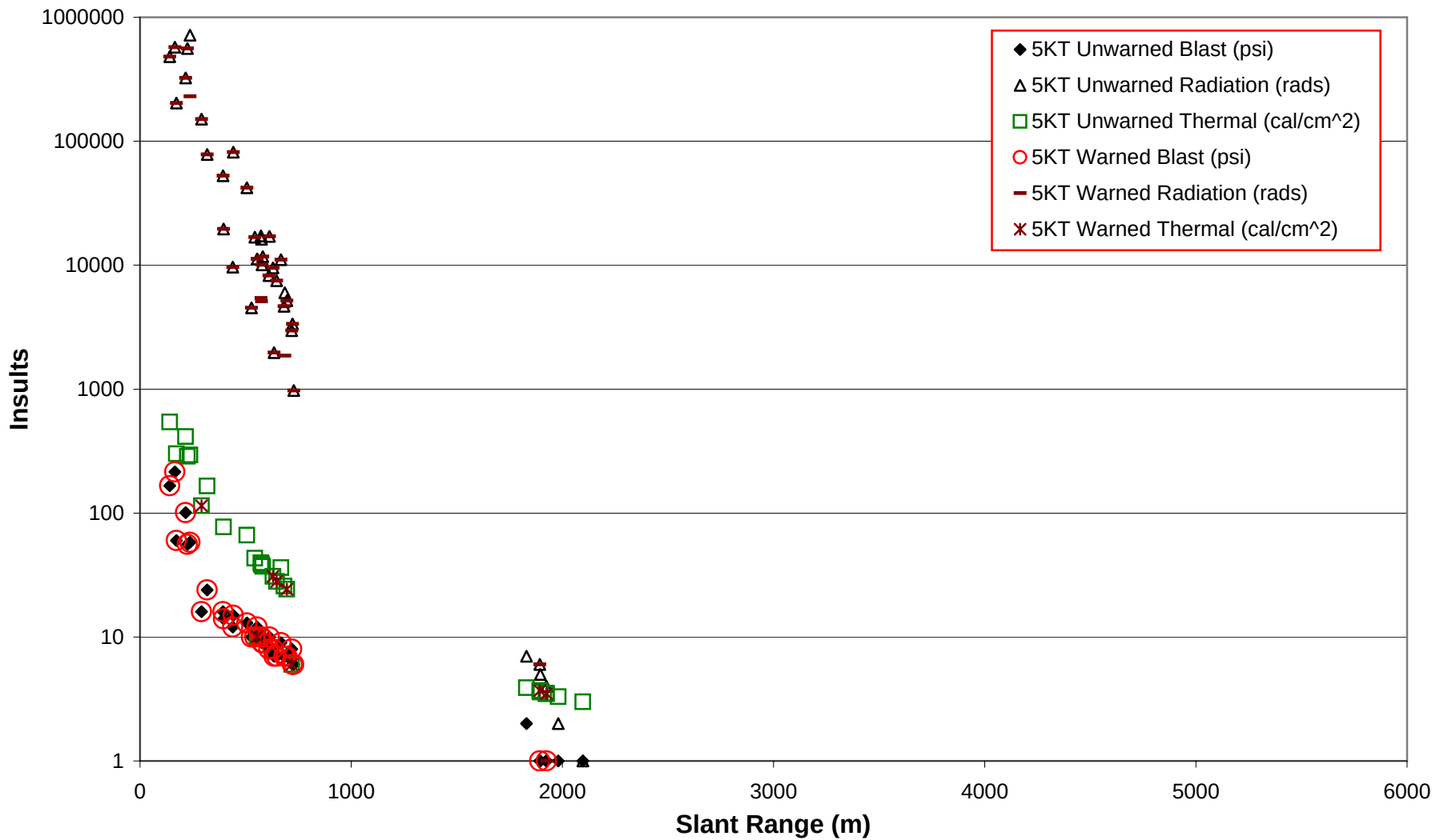
Fig. D2-1 Blast, Radiation, and Thermal Insults- 5KT Heavy Brigade, Forward Maneuver Battalion, Defense
