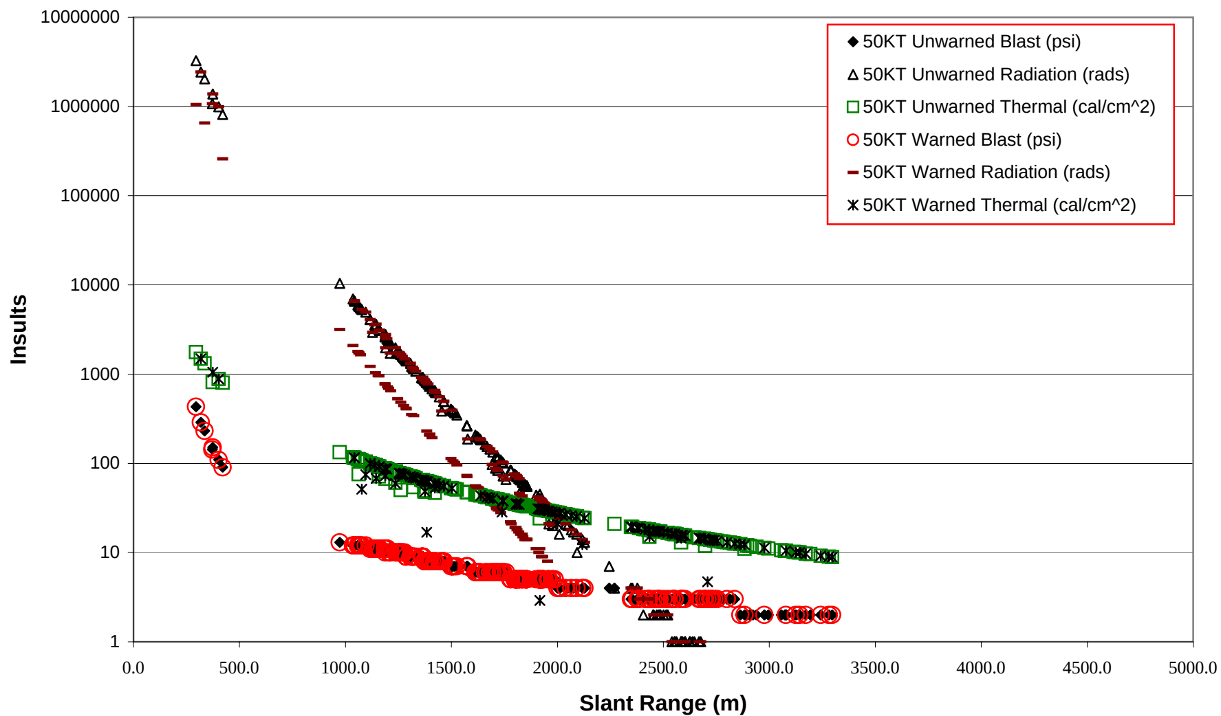
Fig. E2-3 Blast, Radiation, and Thermal Insults- 50KT Heavy Brigade, Brigade Support Area Task Force, Offense and Defense
