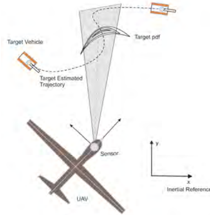
Figure 11: UAV-Sensor-Target Schematic
