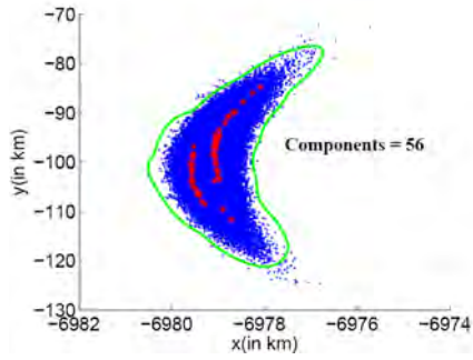
(e) pdf contours in XY plane at 4 hr
