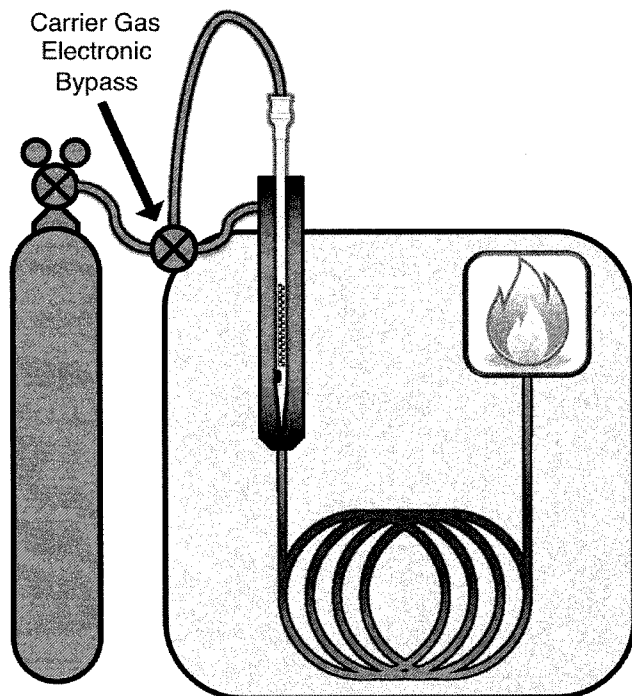
Figure 10. GC-FID with electronic carrier gas bypass
