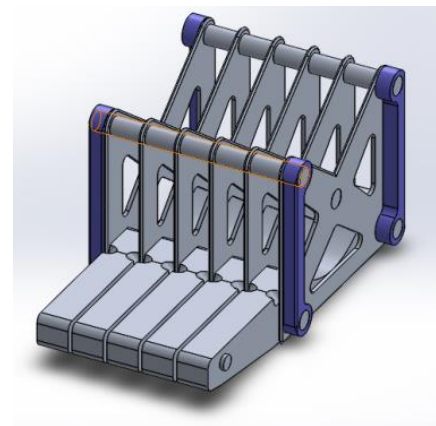
Figure 74: Pulley Lift End Effector
