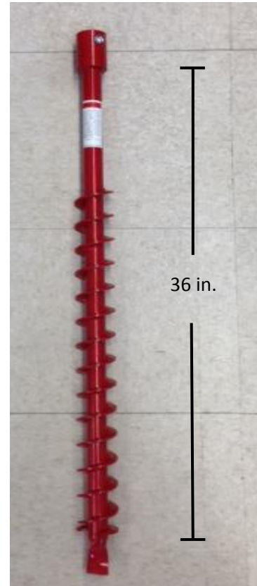
Figure 22: 2" Auger Bit
