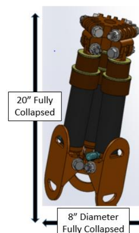
Figure 29: Collapsed Tripod Shoring Solution
