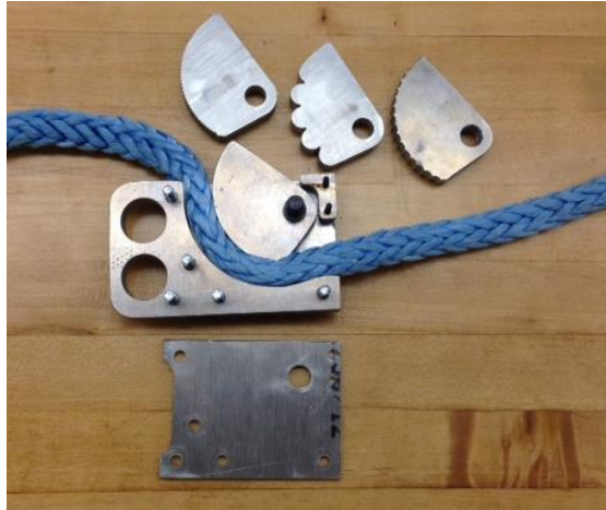
Figure 53: Custom Belay Device
