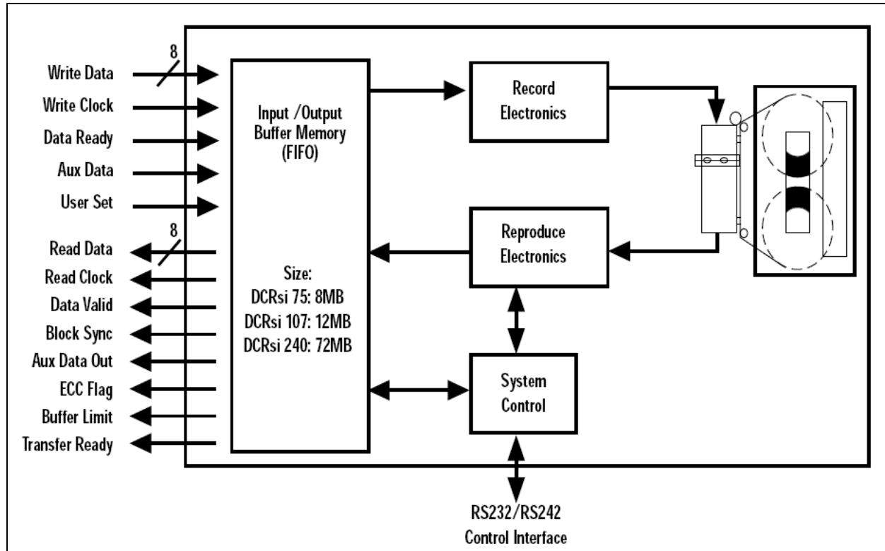
Figure 5-53. Ampex DCRsi Interface
