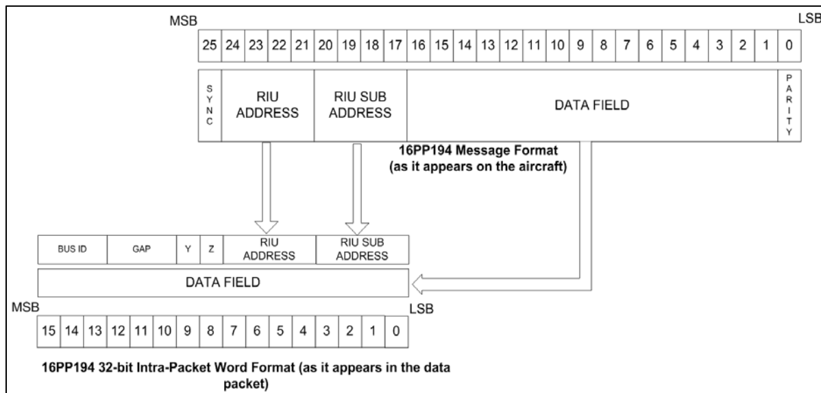
Figure 5-31. 16PP194 to IRIG 106 Chapter 10 Data Bit Mapping
