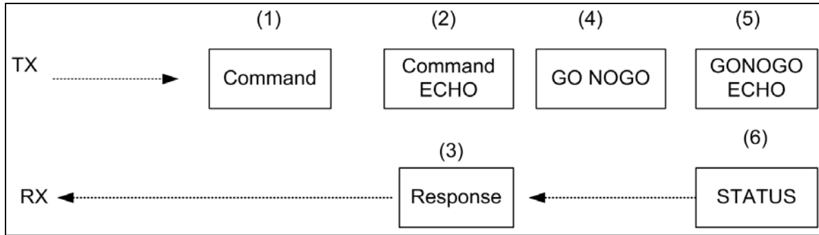
Figure 5-29. 16PP194 Message Transaction
