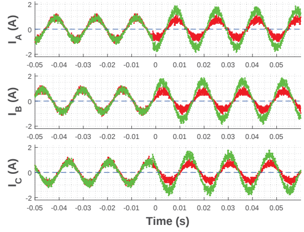
(b) The load carried by one inverter is decreased by increasing virtual output impedance
