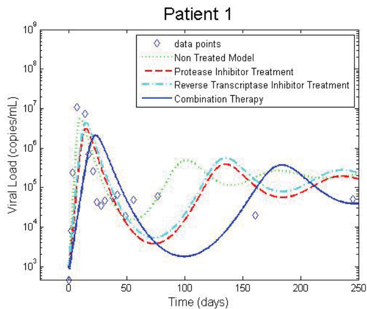
Figure 47: The increased impact of combination therapy with both inhibitors at 0.3.
