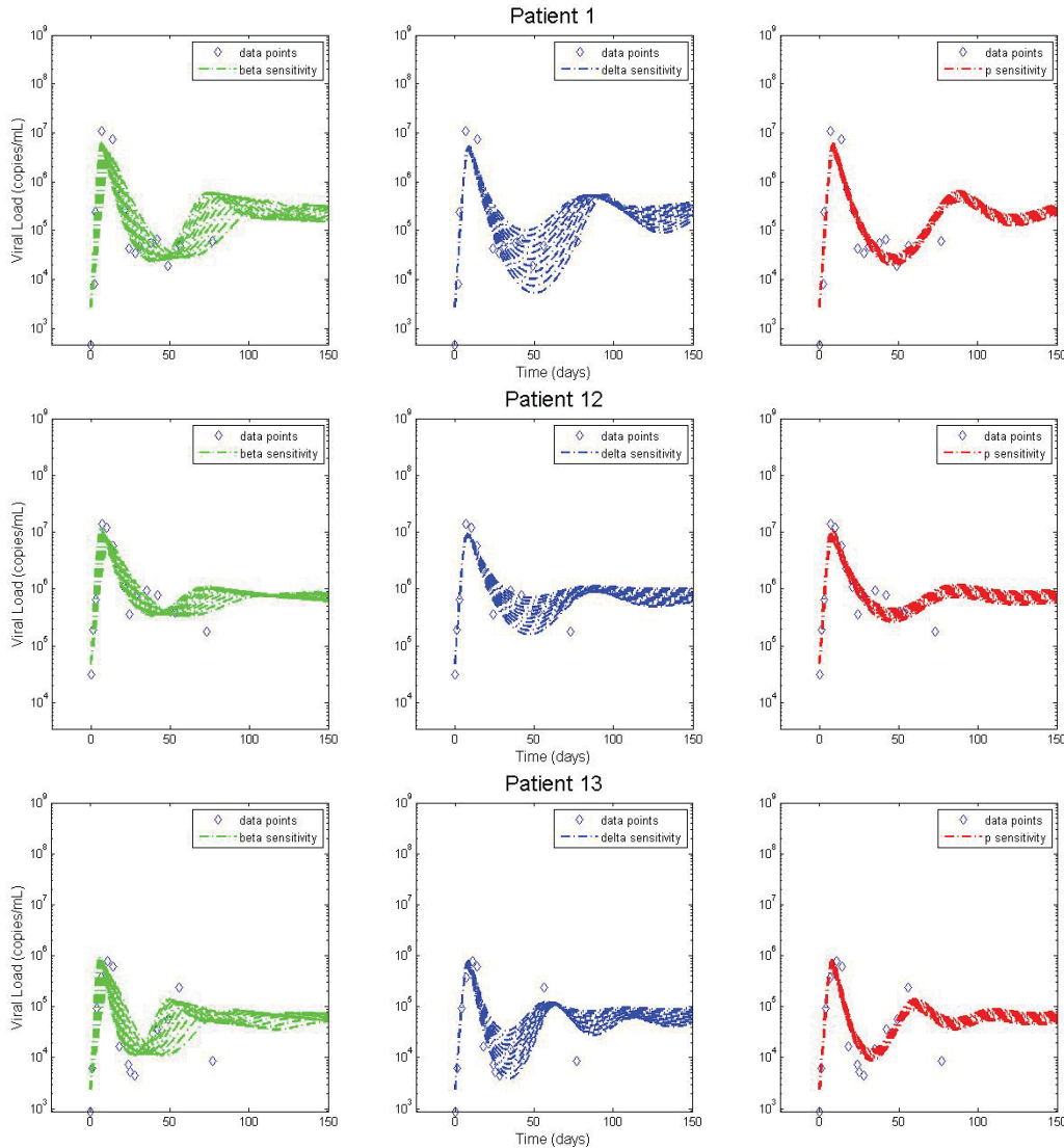
Figure 26: The effect of varying the parameters \beta , \delta , and p .
