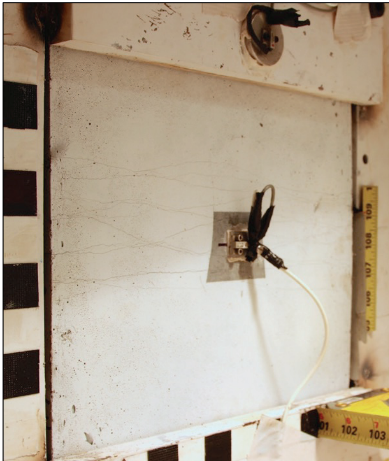
Figure 6.10. Small-scale BLS test setup showing accelerometer positions and scales used for high-speed video measurements.
