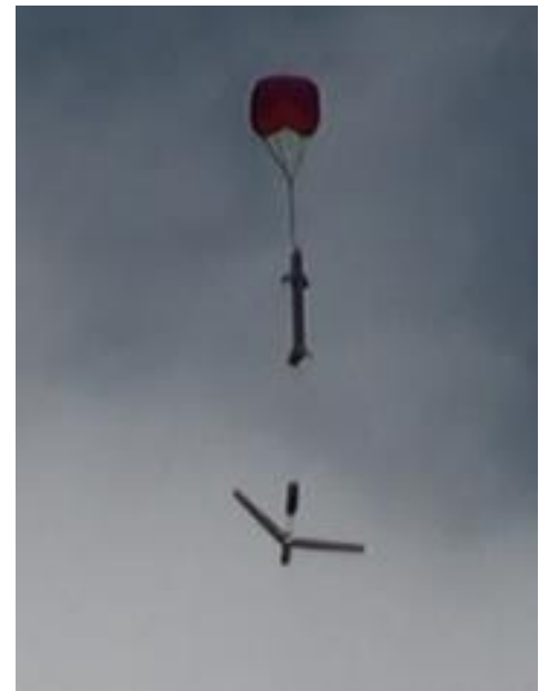
Figure 14: After GliderSonde has been ejected from the tube, its wings are unfolded while still tethered and descending slowly on the parachute.
