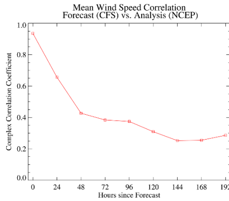
Figure 7 Correlation coefficient between wind velocity between CFS-V2 forecast and NCEP/NCAR reanalysis.
