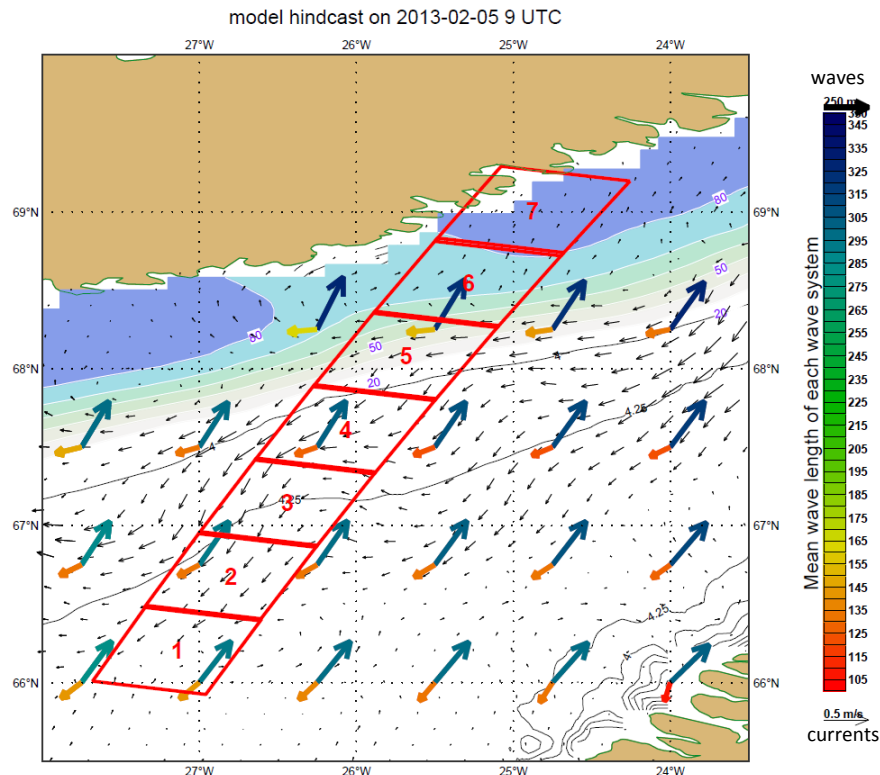
Figure 1: WAM hindcast underlying a TerraSAR-X stripmap for swell penetrating into the East Greenland sea ice
