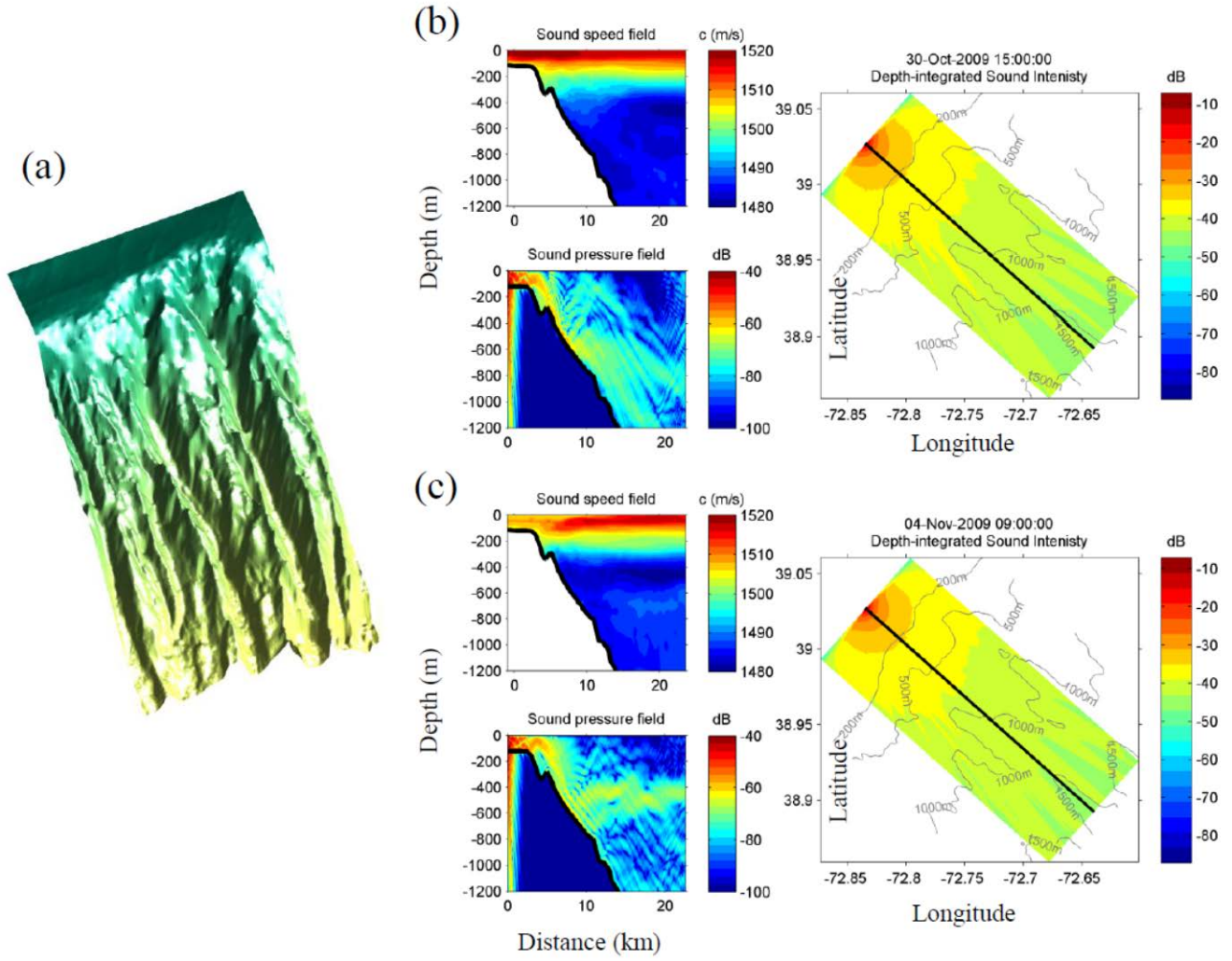
Figure 2: Integrated numerical simulations of ocean dynamics and acoustics on the slope of the New Jersey Shelf. [(a)The bathymetry, (b) the original down-slope propagation pattern, and (c) change of propagation pattern to water-borne ducting due to water column variability. The beam pattern on the depth integrated sound intensity plots on the right shows the 3-D focusing of sound by the small canyons on the slope.]
