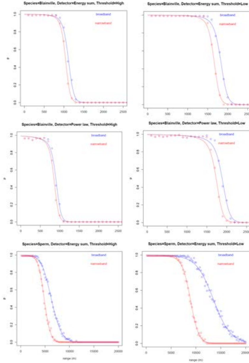
Figure 4. Detection functions of simulated echolocation clicks added to background noise for different species and detectors. Circles indicate probabilities of detections obtained by modeling the propagation loss using a broadband approximation (blue), and narrowband approximation (red). Solid lines indicate fits of detection functions, used to measure the effective detection ranges and areas. Top: Detection function of a single on-axis Mesoplodon densirostris (Blainville's beaked whale) click using a simple energy detector (with DT=7 dB) corresponding to a FAR = 10/h , and DT = 3 dB, corresponding to a FAR \sim 200/h ). Middle: Detection of a Blainville's beaked whale click using a power law Page test detector (with DT = 12 dB) corresponding to a FAR = 1/h , and DT = 2 dB, corresponding to a FAR \sim 200/h ). Bottom: Detection function of a single on-axis Physeter macrocephalus (sperm whale) click using a simple energy detector (with DT = 23 dB, corresponding to a FAR = 1/h , and with DT = 11 dB, corresponding to a FAR = 200/h ). Note that variance estimates were omitted. A system-noise limited background noise was adopted for this example (see von Benda-Beckmann et al. 2010).
