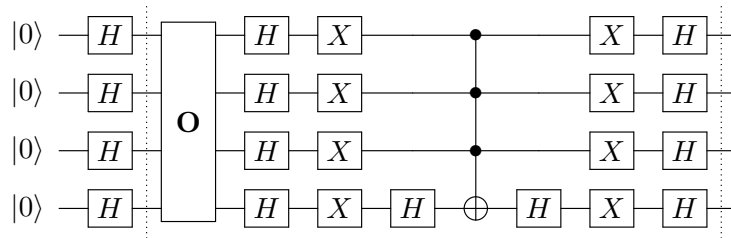
Figure 6.2: A quantum circuit to perform Grover's algorithm with 4 qubits. The dotted lines enclose the Grover iteration, which must be repeated multiple times to obtain the solution with a high probability.
