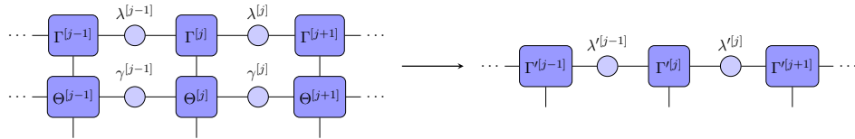
Figure 3.12: The application of a MPO to a MPS.
